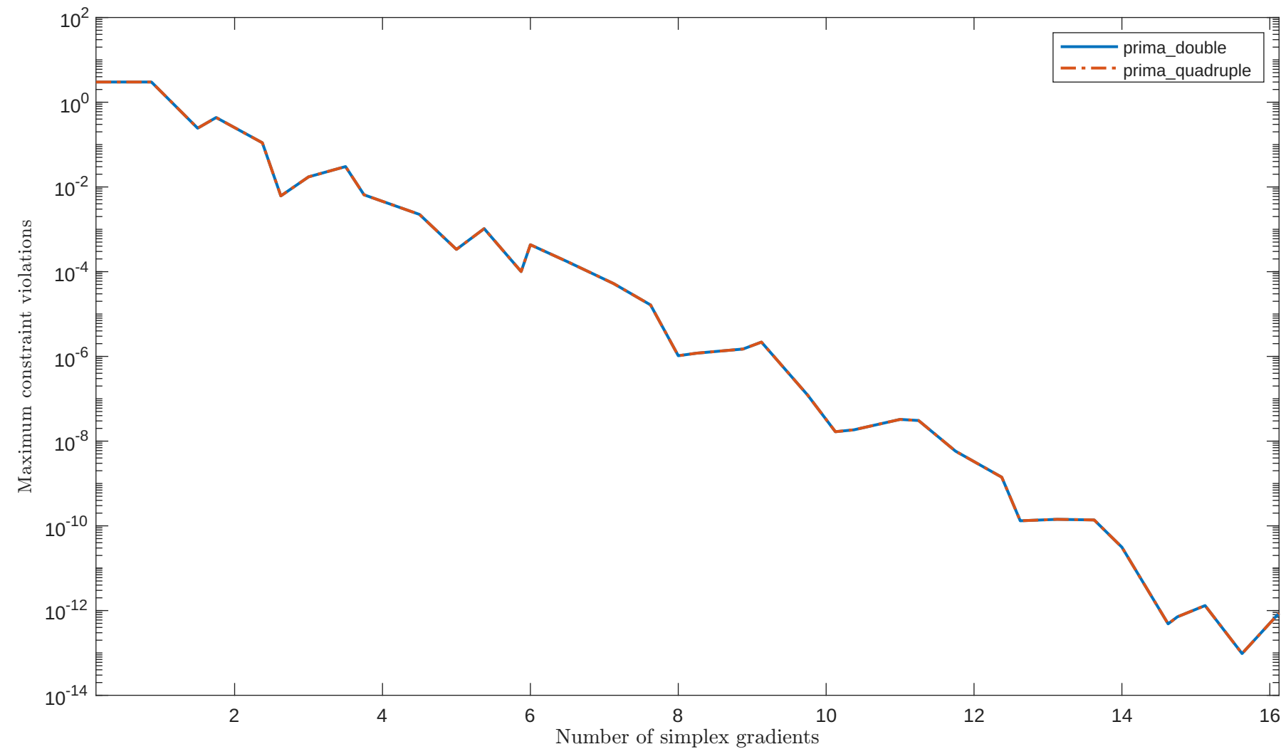
Solving "LUKVLE12" with "plain" feature
