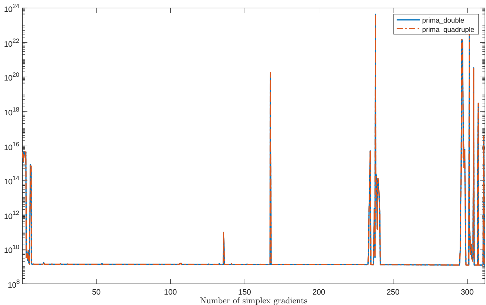
Solving “MGH10LS” with “plain” feature
