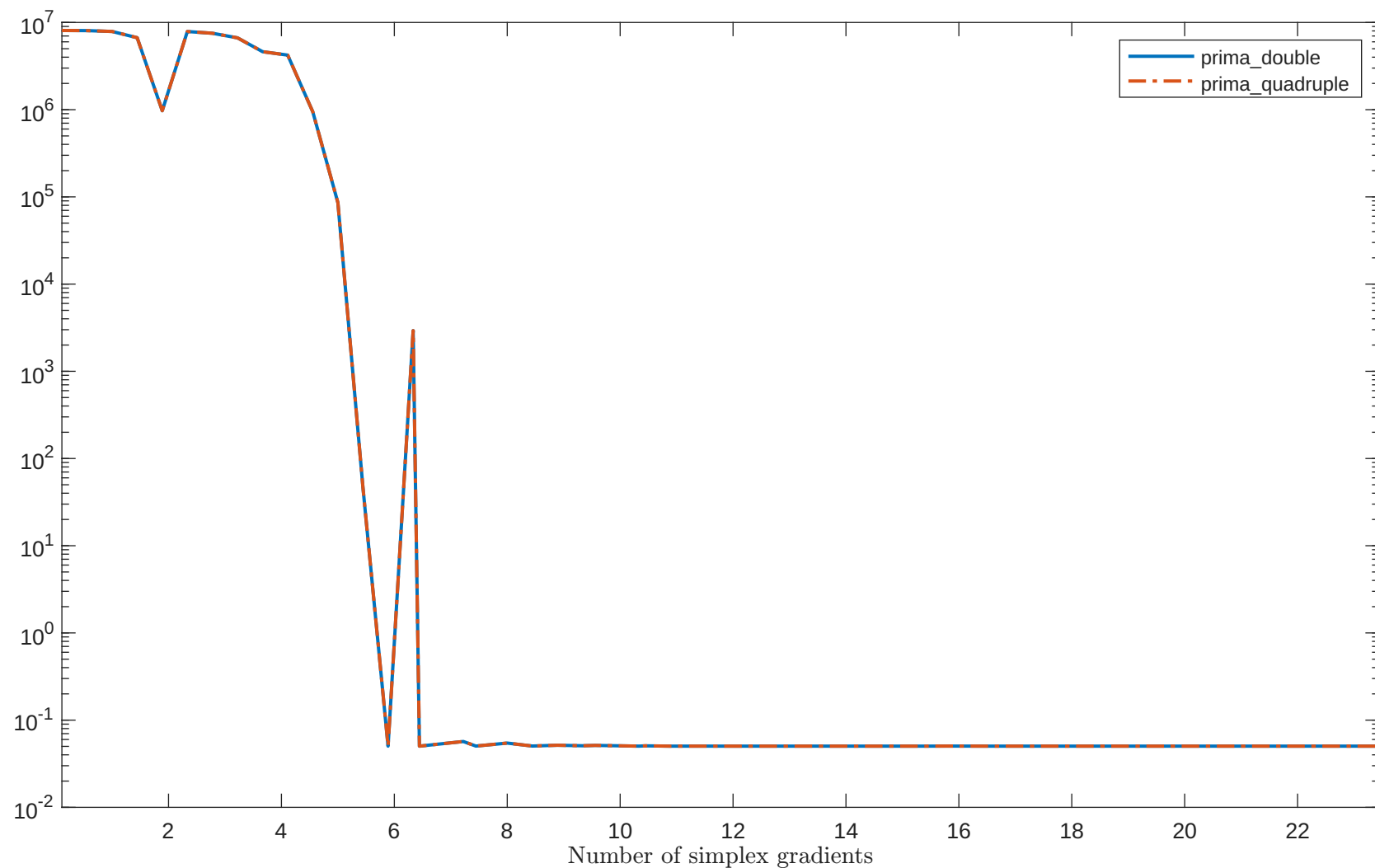
Solving "PALMER4C" with "plain" feature
