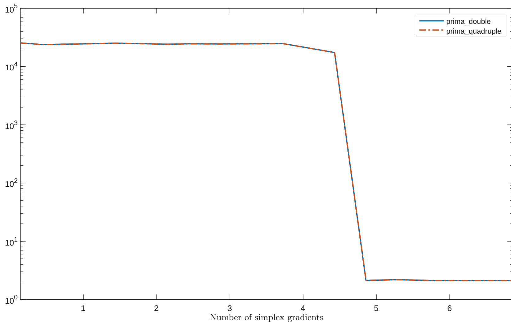
Solving "PALMER5C" with "plain" feature
