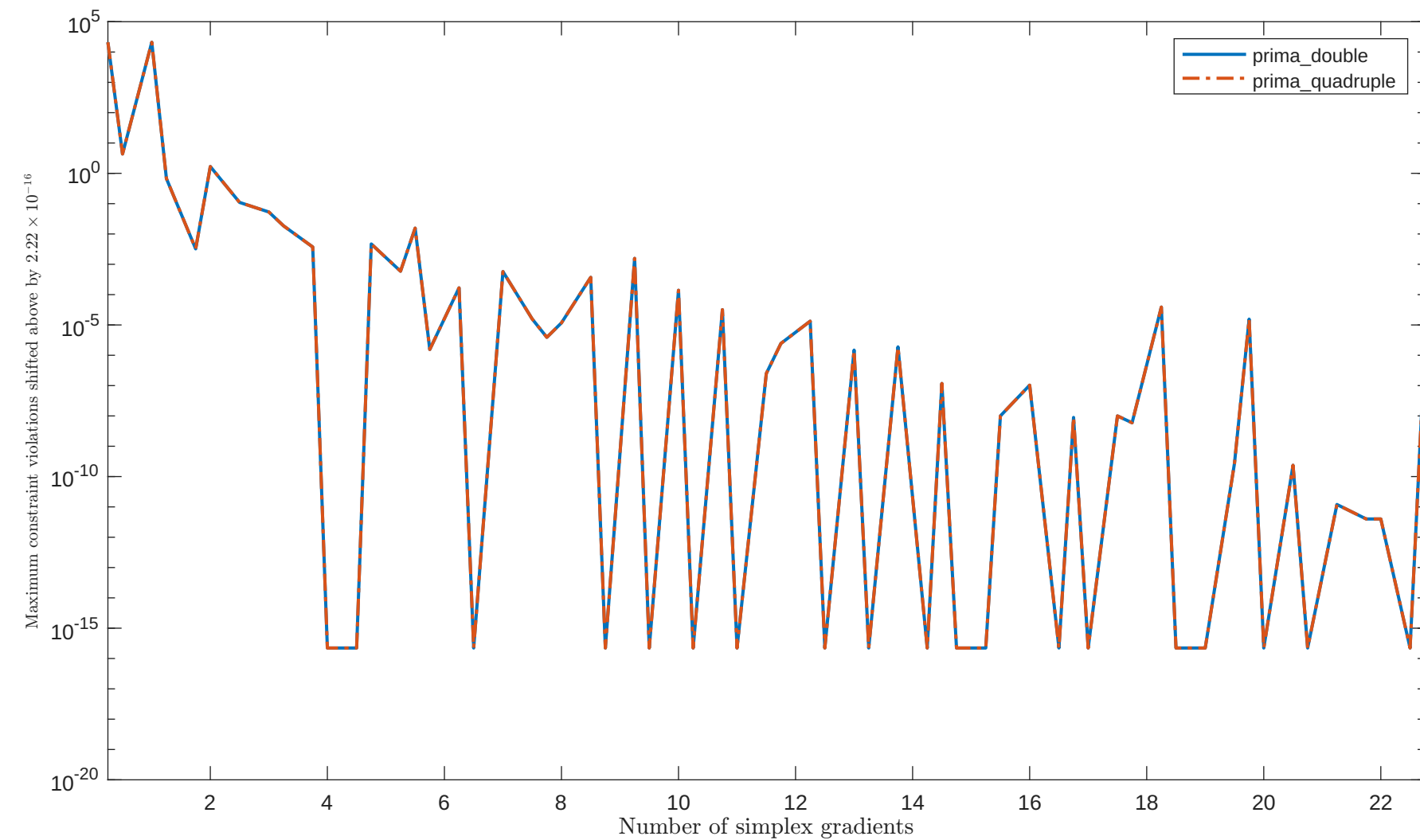
Solving "POLAK4" with "plain" feature
