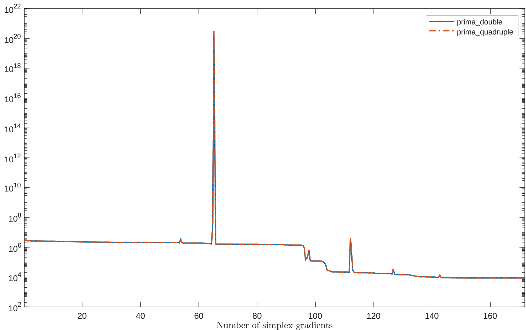
Solving "RAT43LS" with "plain" feature
