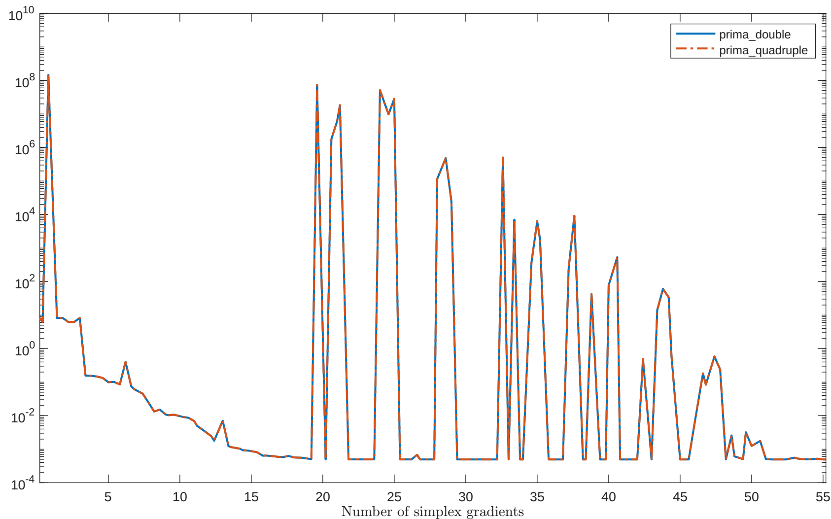
Solving "ROSZMAN1LS" with "plain" feature
