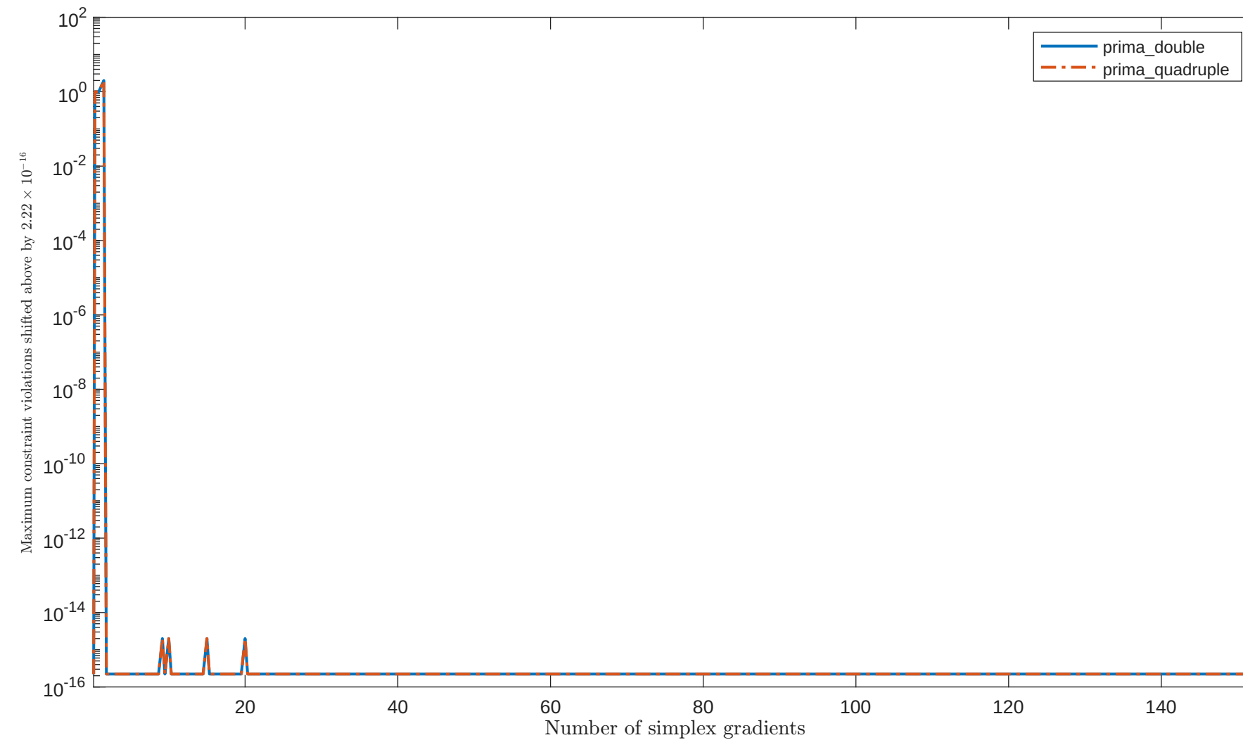
Solving "S268" with "plain" feature
