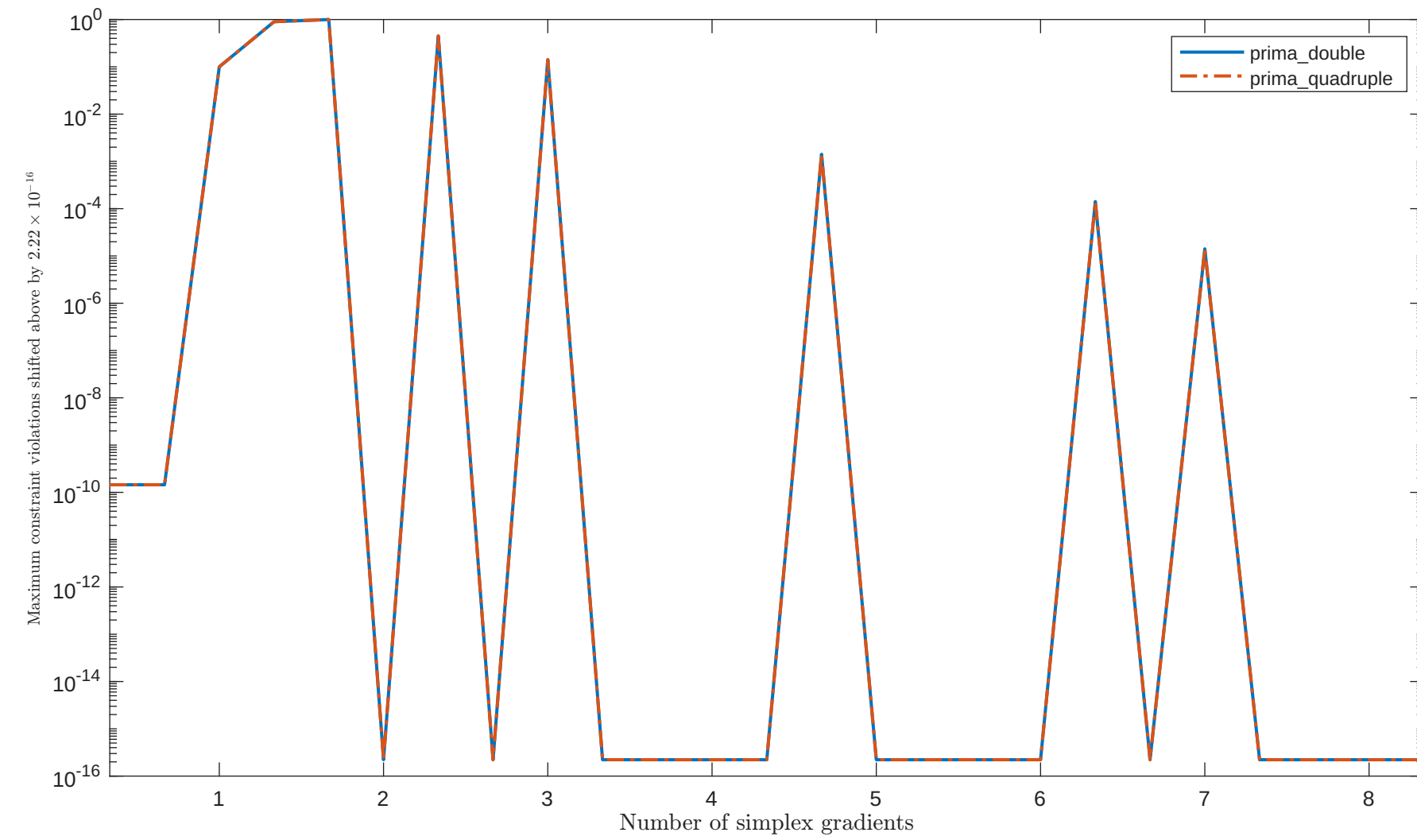
Solving "ZECEVIC2" with "plain" feature
