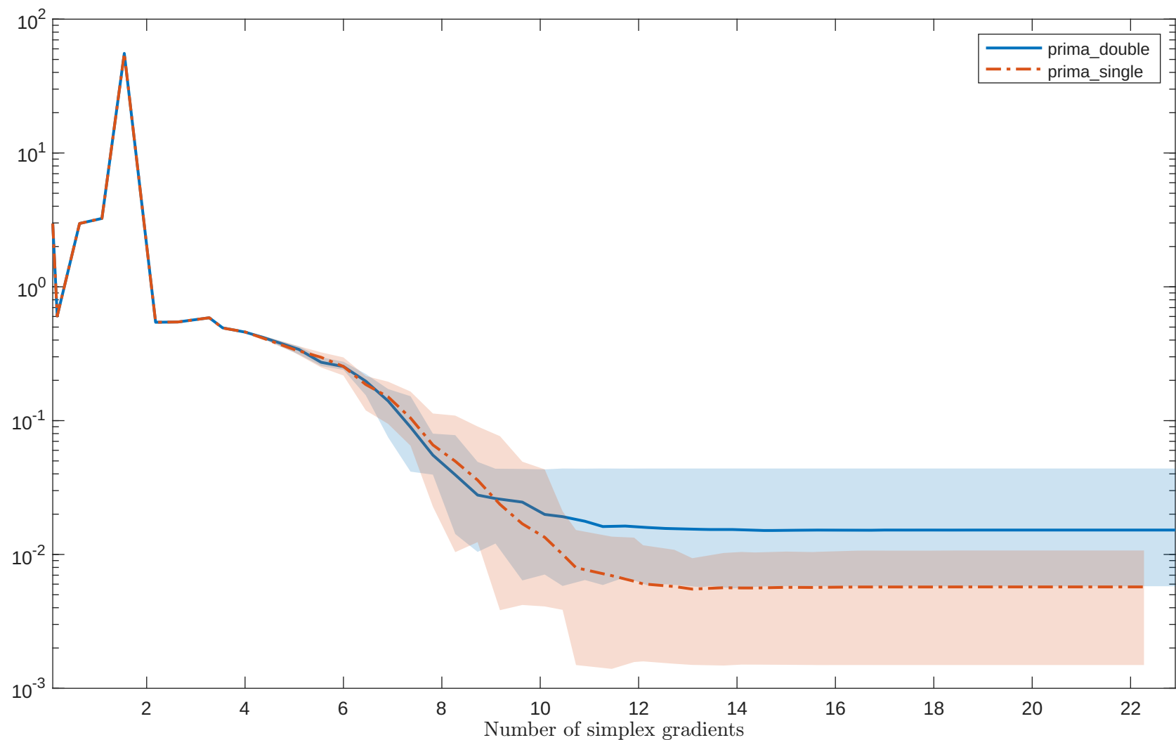
Solving "ARGTRIGLS" with "noisy_0.001_mixed_gaussian" feature
