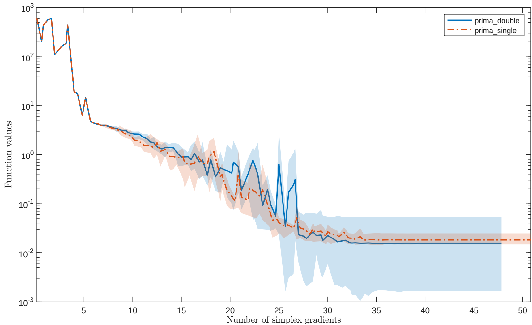
Solving “CHNRSNB” with “noisy_0.001_mixed-gaussian” feature
