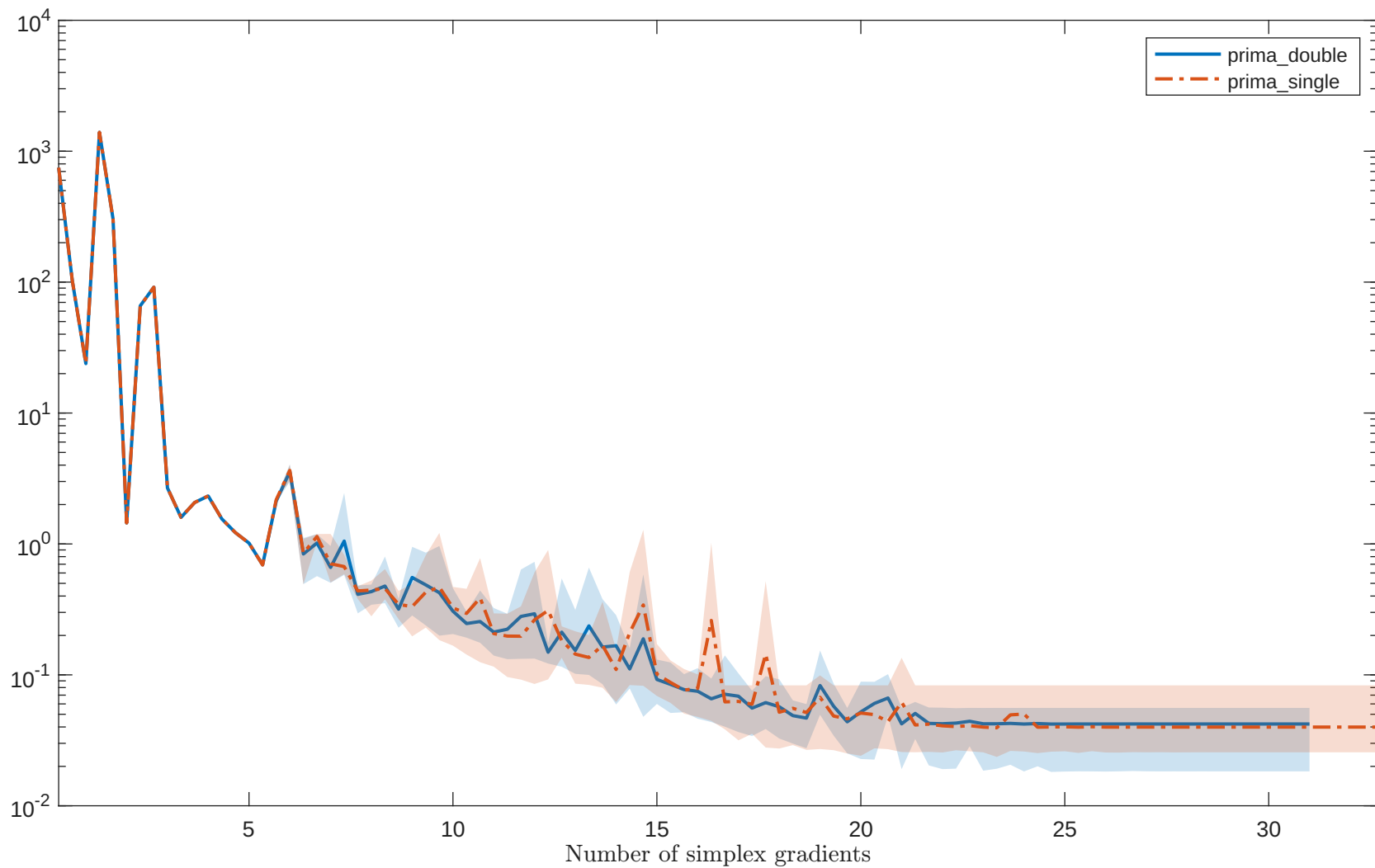
Solving “CUBE” with “noisy_0.001_mixed_gaussian” feature
