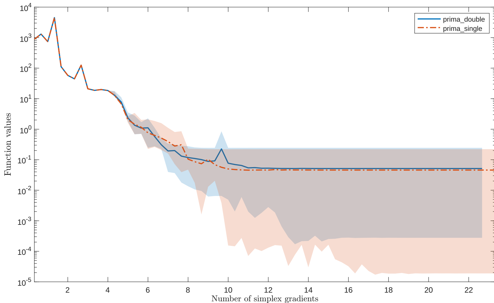
Solving "DENSCHNC" with "noisy_0.001_mixed-gaussian" feature
