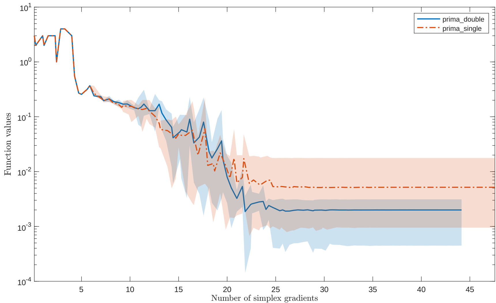
Solving “EIGENBLS” with “noisy_0.001_mixed_gaussian” feature
