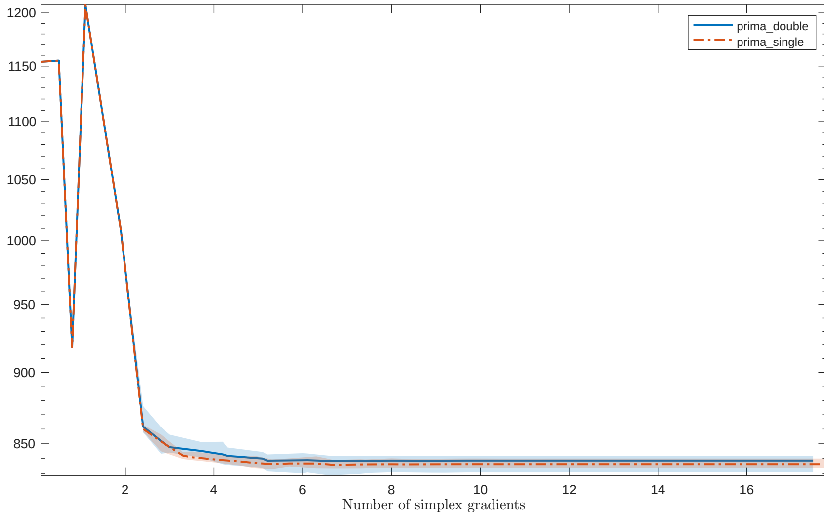
Solving “ENSOLS” with “noisy_0.001_mixed_gaussian” feature
