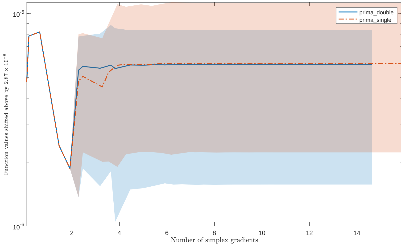
Solving “FLETCBV3” with “noisy_0.001_mixed_gaussian” feature
