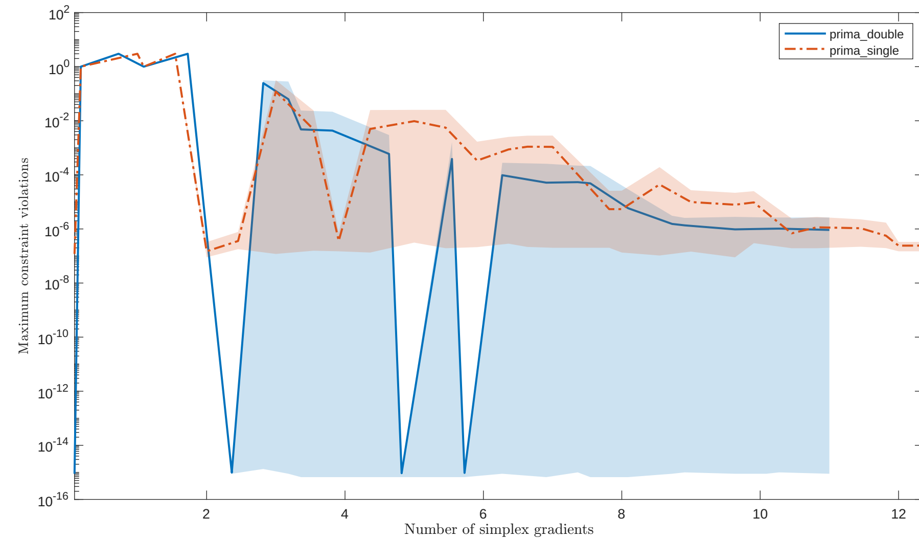
Solving "GENHS28" with "noisy_0.001_mixed-gaussian" feature
