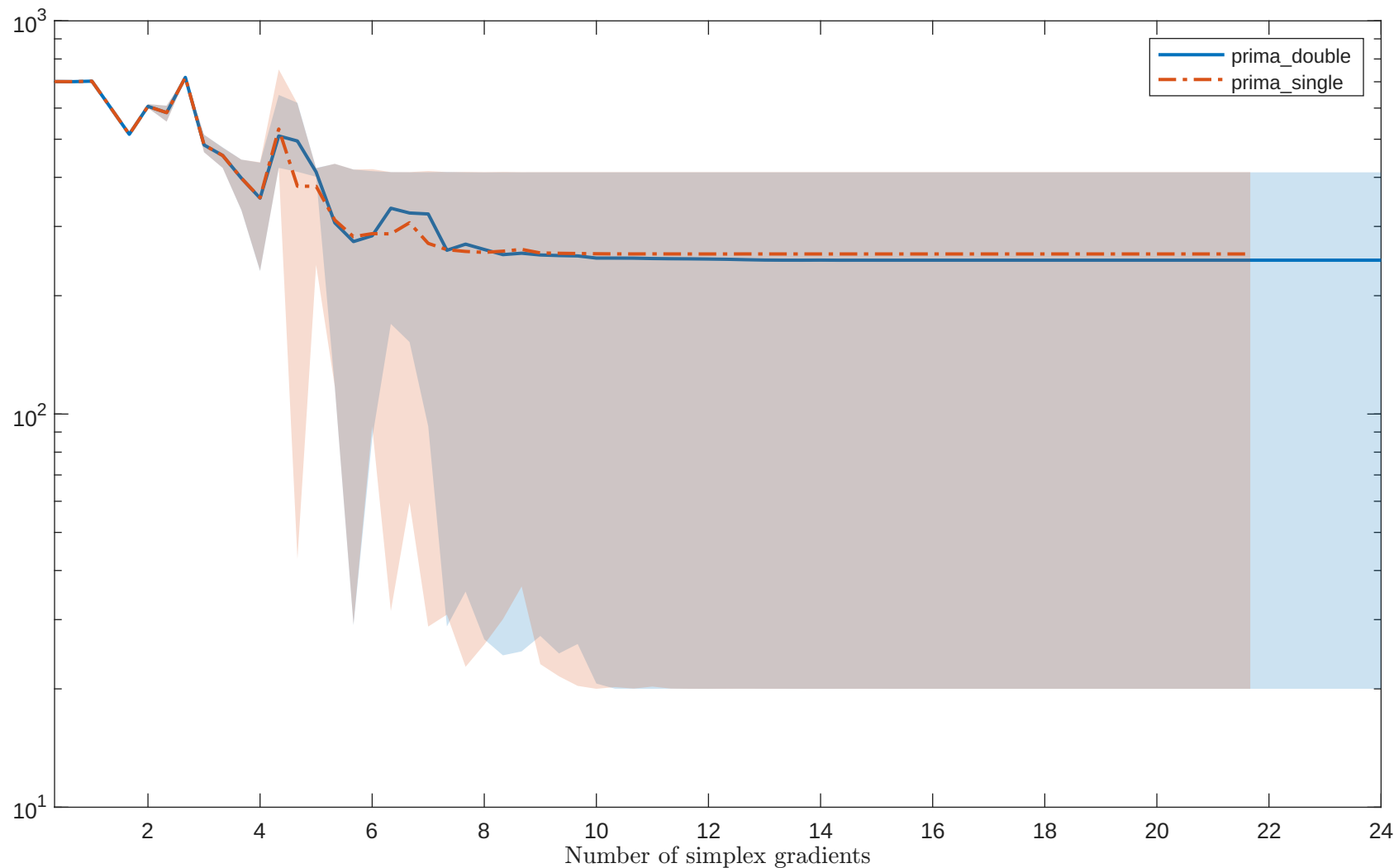
Solving "HAIRY" with "noisy_0.001_mixed_gaussian" feature
