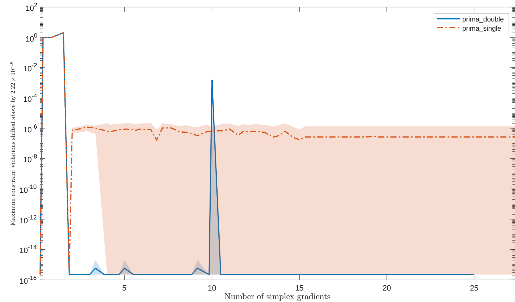
Solving "HS268" with "noisy_0.001_mixed_gaussian" feature
