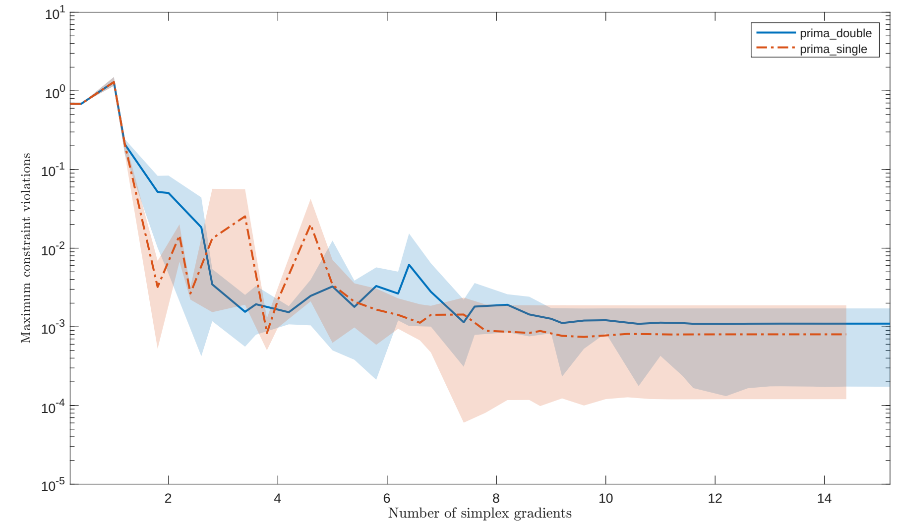
Solving “HS69” with “noisy_0.001_mixed.gaussian” feature
