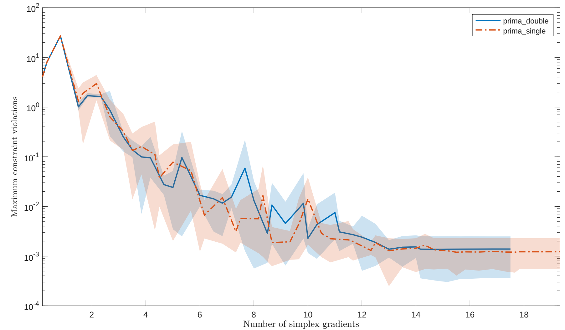
Solving “HS81” with “noisy_0.001_mixed_gaussian” feature
