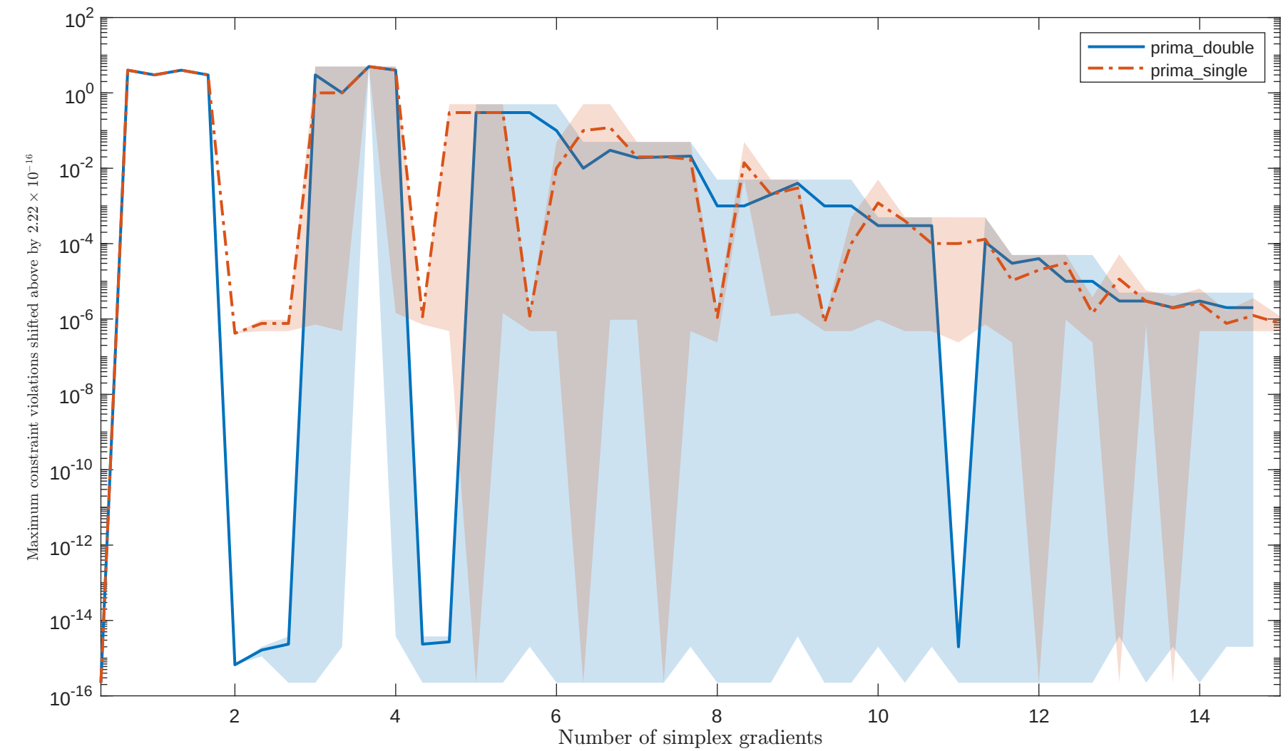
Solving "HS9" with "noisy_0.001_mixed_gaussian" feature
