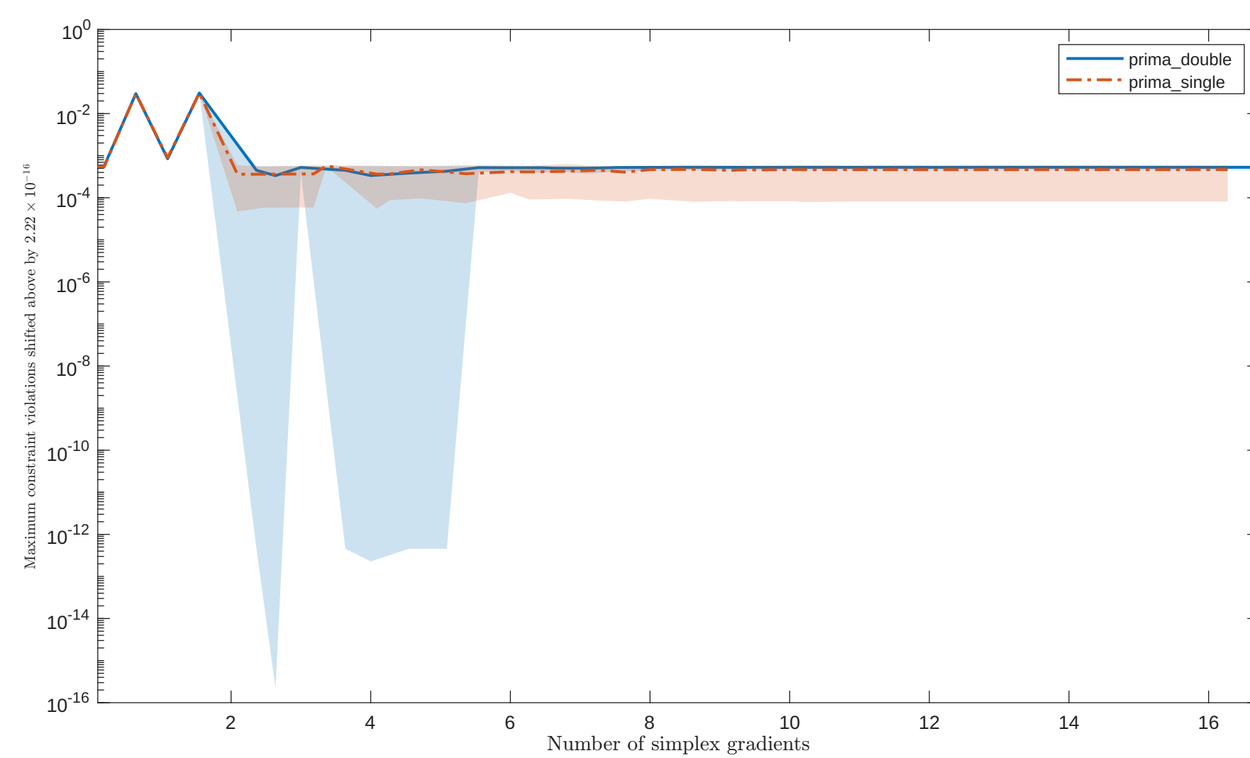
Solving "HUESTIS" with "noisy_0.001_mixed-gaussian" feature
