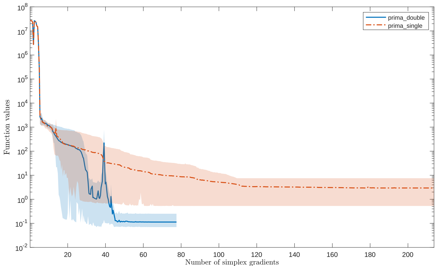
Solving "PALMER2C" with "noisy_0.001_mixed_gaussian" feature
