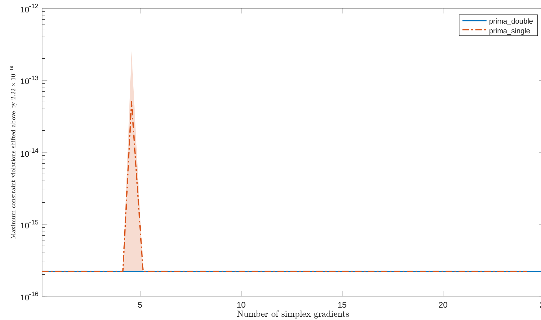
Solving “PALMER4A” with “noisy_0.001_mixed_gaussian” feature
