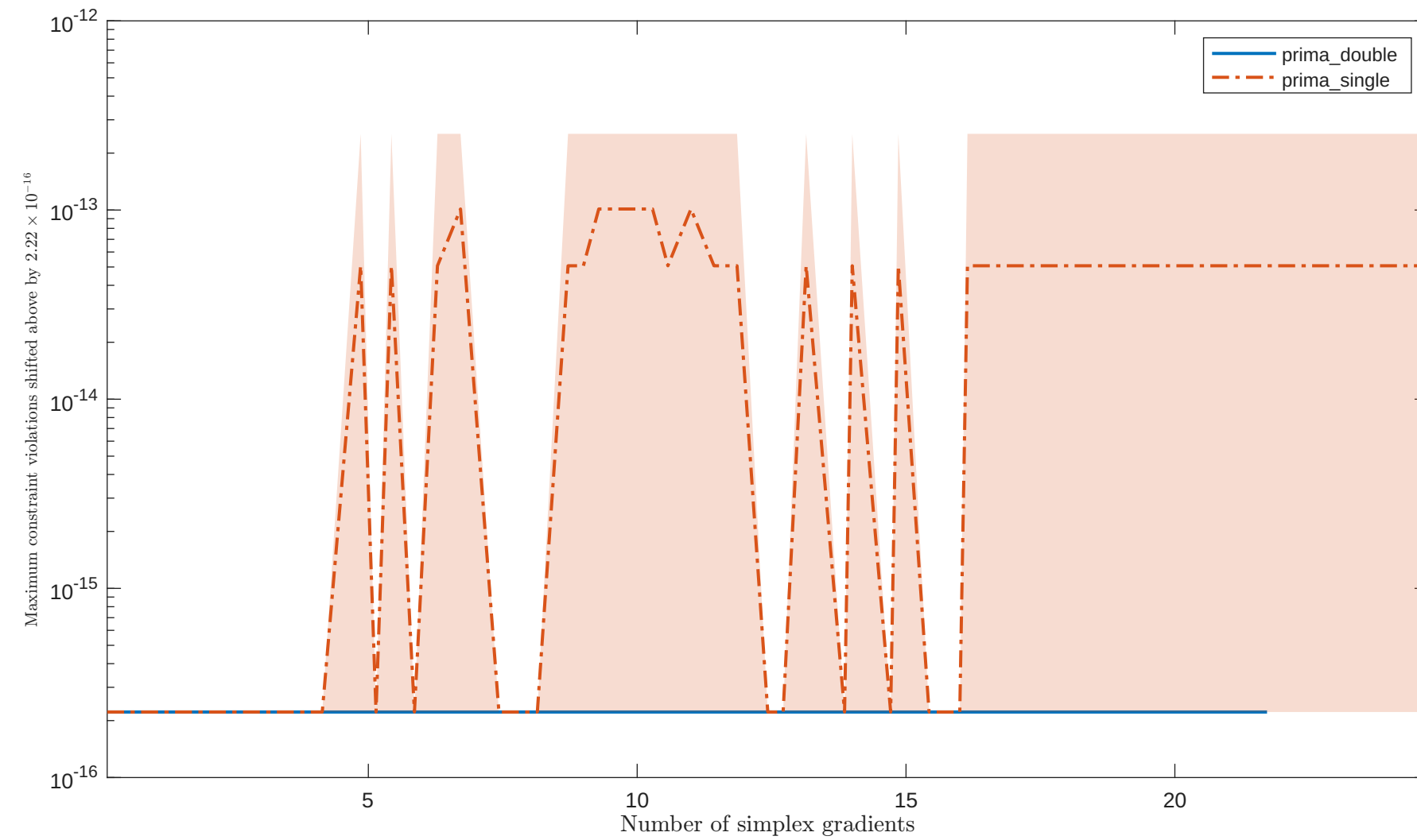
Solving "PALMER7A" with "noisy_0.001_mixed_gaussian" feature
