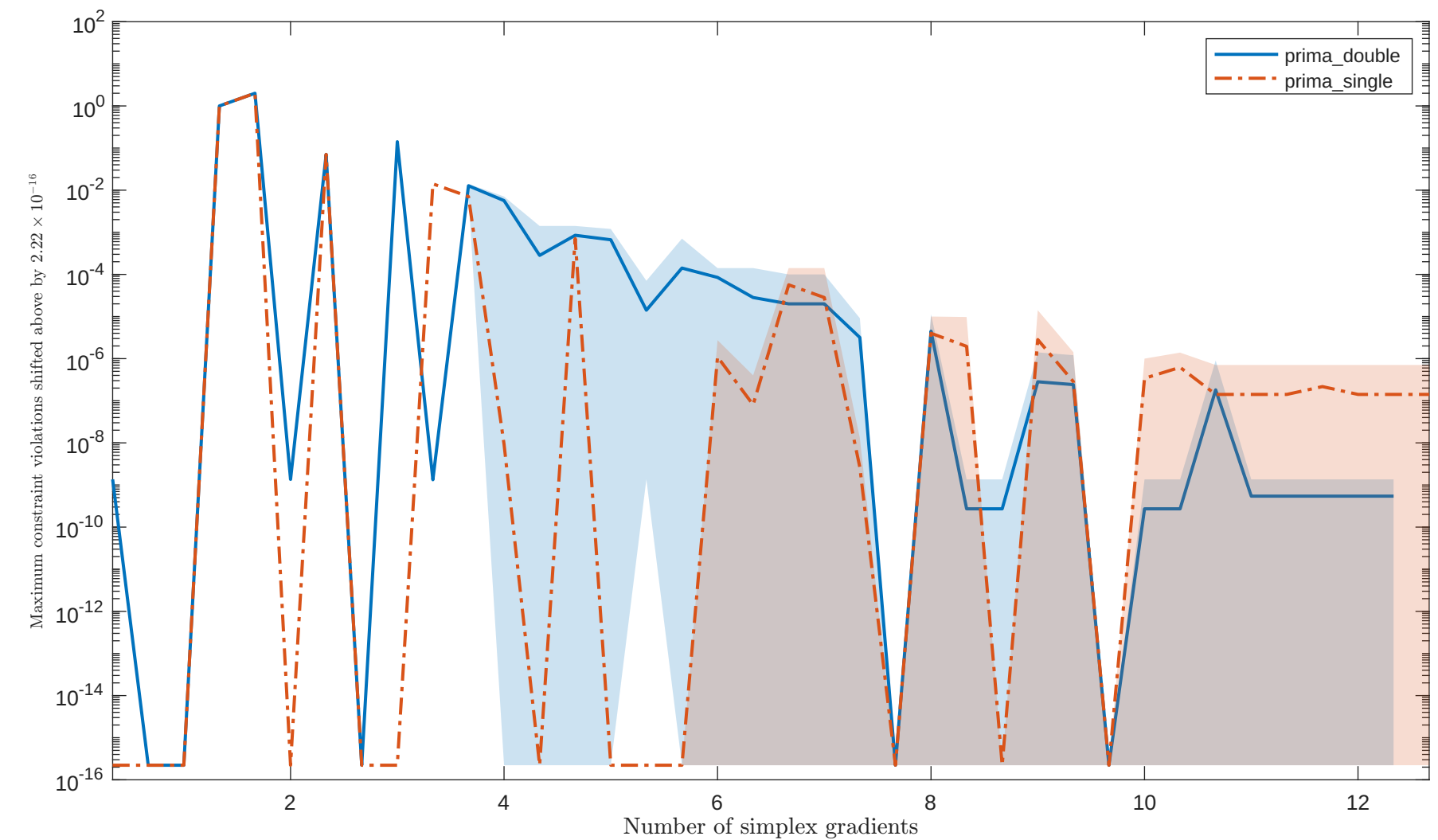
Solving "SIMPLLP" with "noisy_0.001_mixed_gaussian" feature
