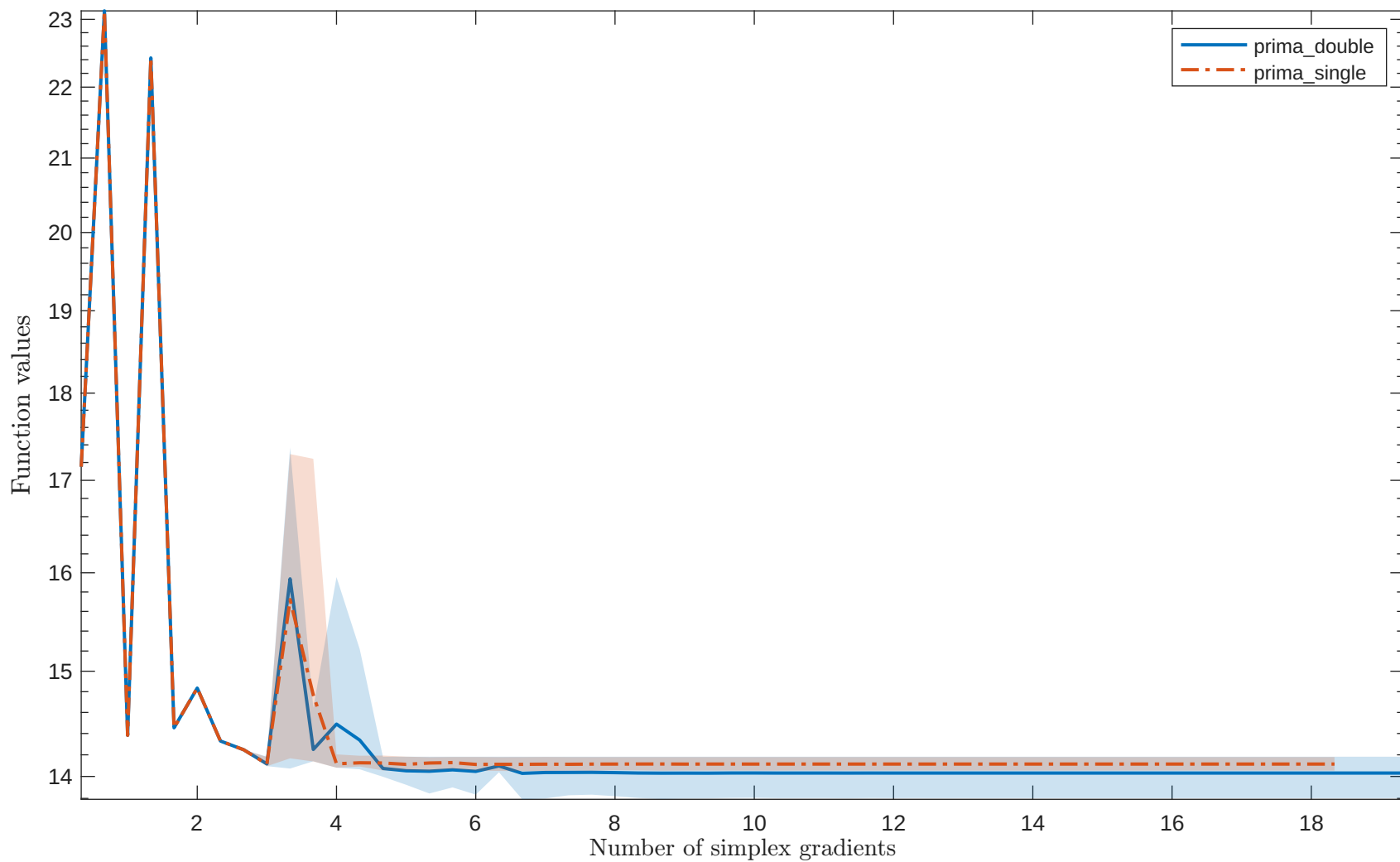
Solving “SNAIL” with “noisy_0.001_mixed_gaussian” feature
