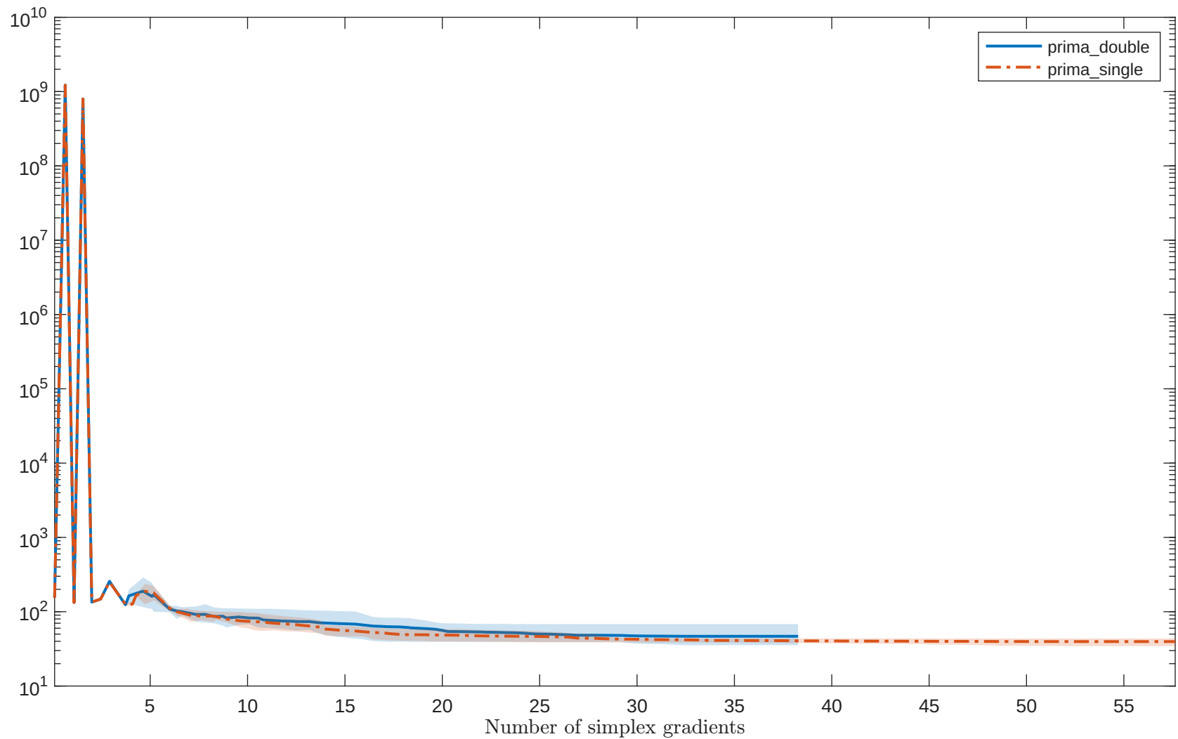
Solving “SSBRYBND” with “noisy_0.001_mixed_gaussian” feature
