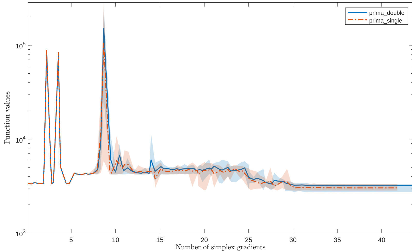
Solving “VESUVIALS” with “noisy_0.001_mixed_gaussian” feature
