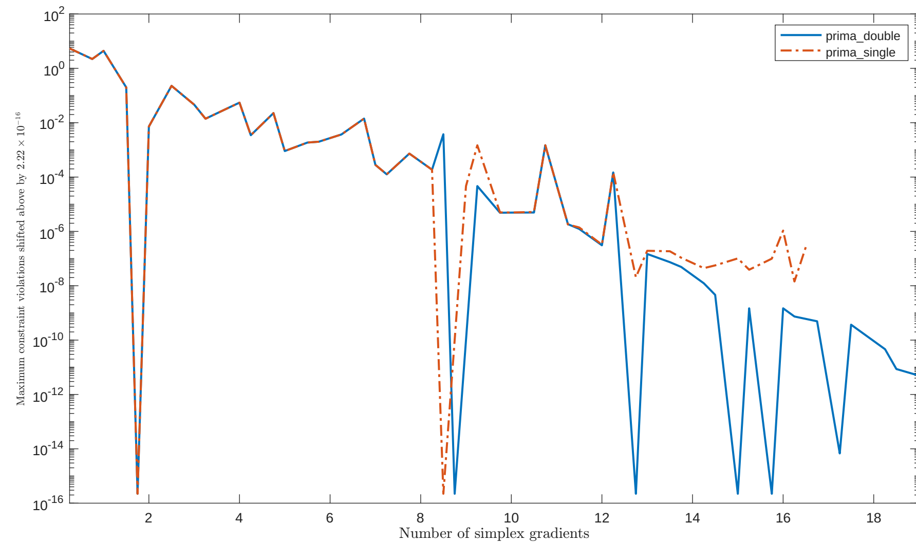
Solving "CHACONN1" with "plain" feature
