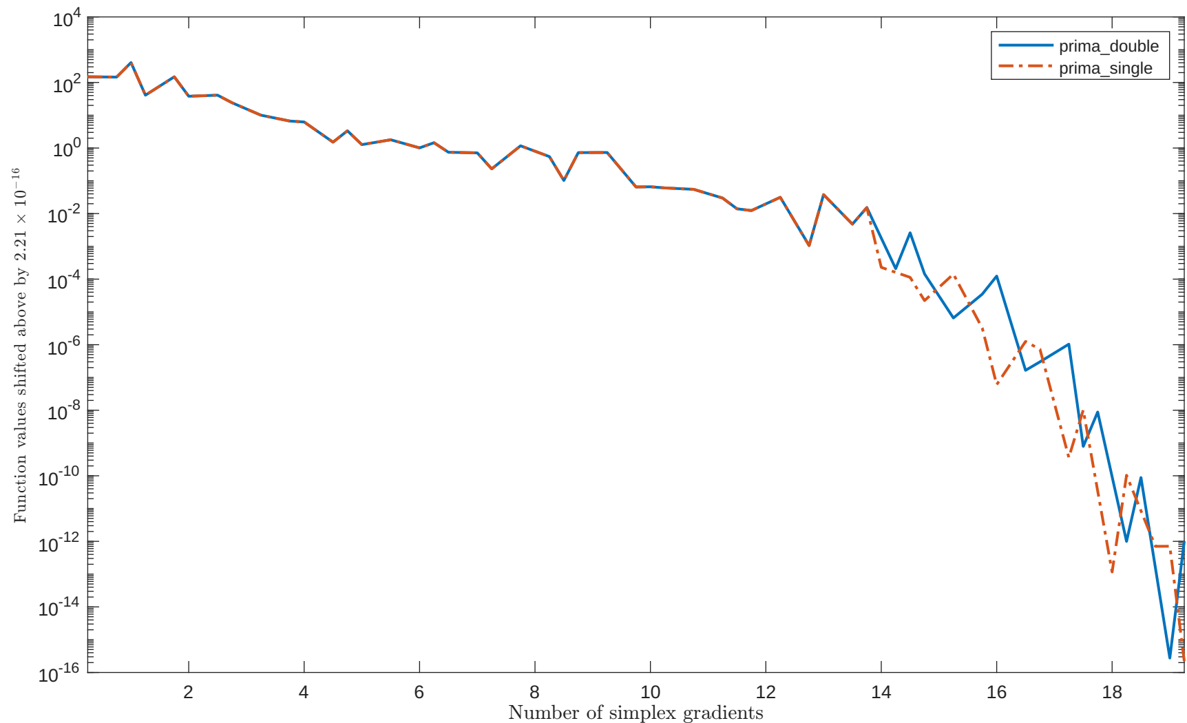
Solving "DENSCHNE" with "plain" feature
