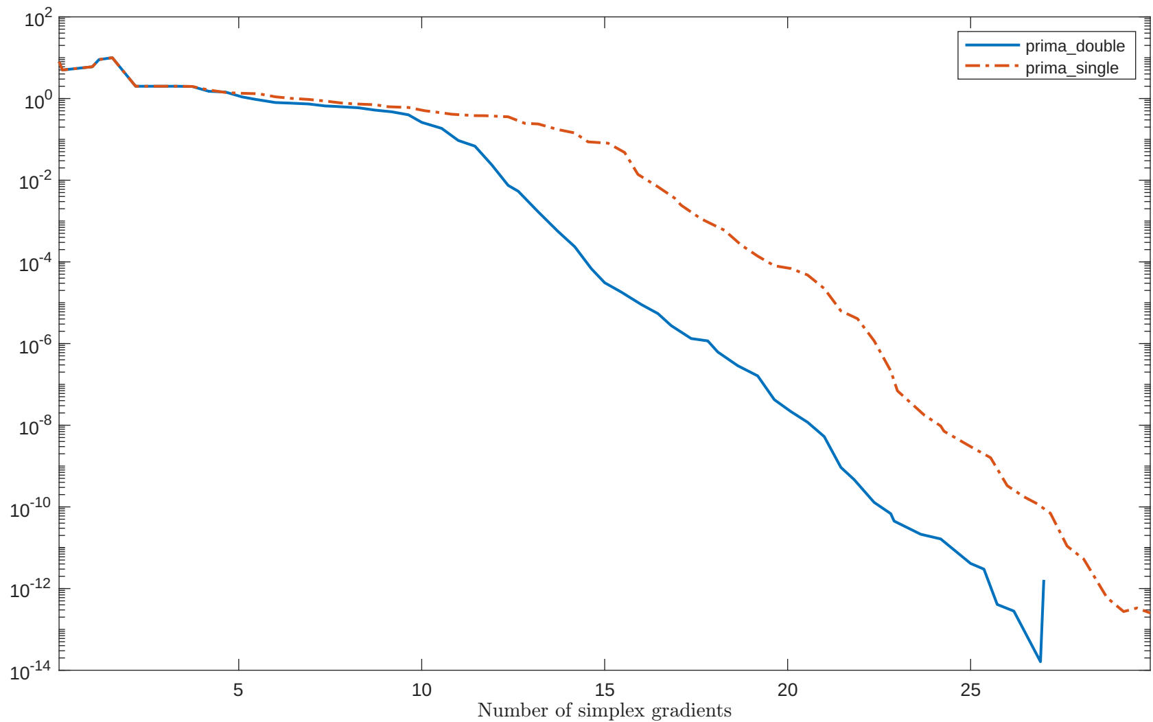
Solving "DIXON3DQ" with "plain" feature
