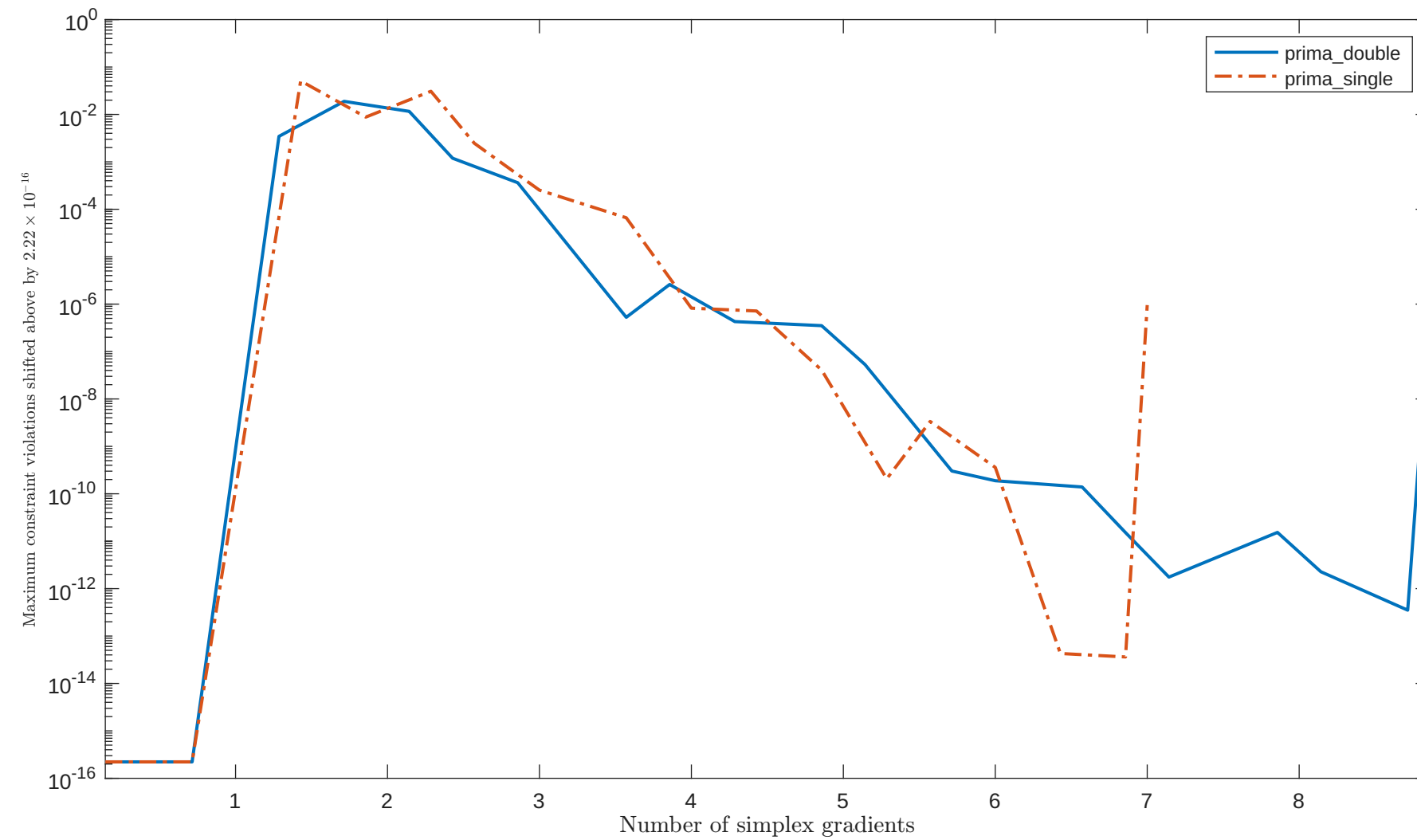
Solving "EIGENBCO" with "plain" feature
