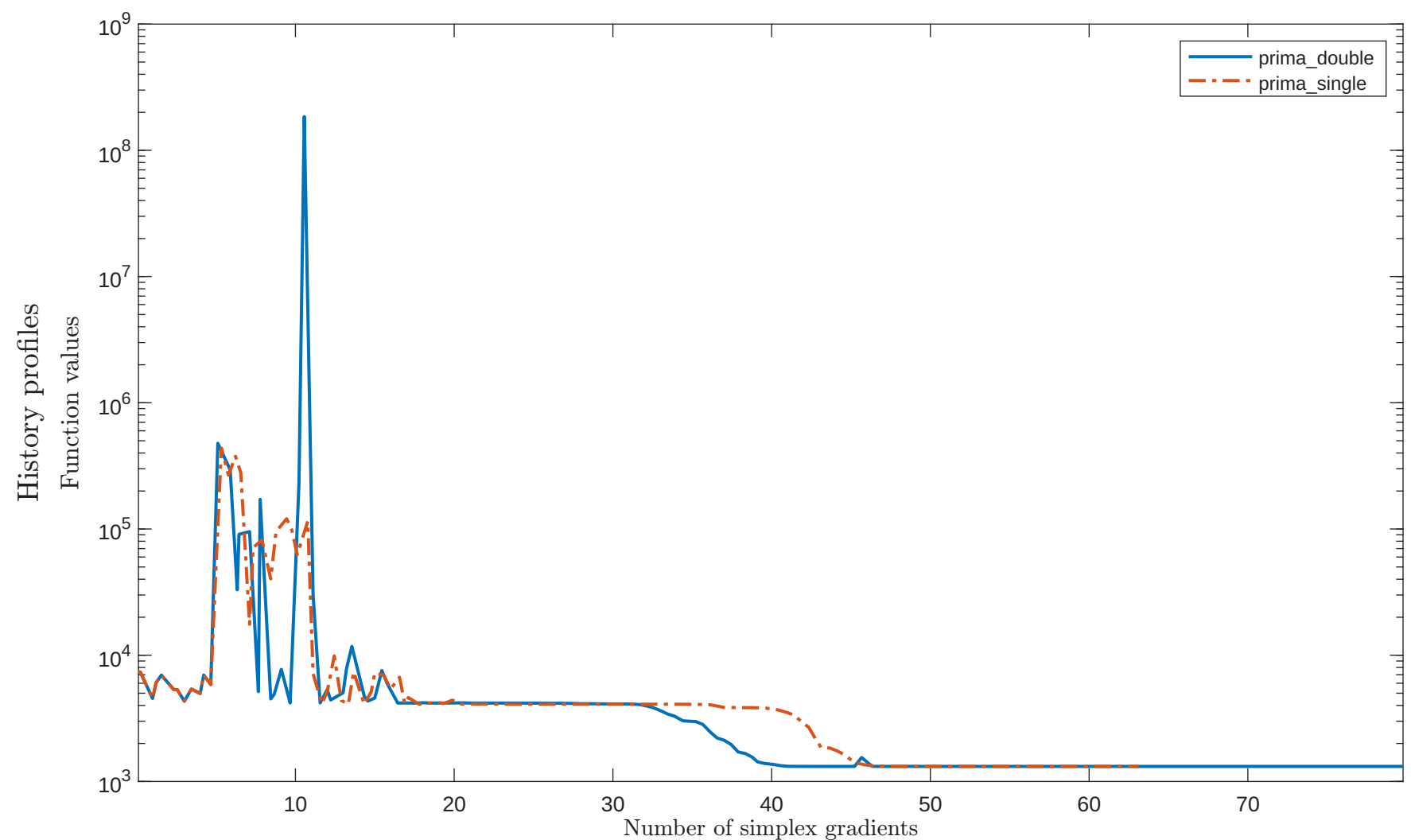
Solving “GAUSS1LS” with “plain” feature
