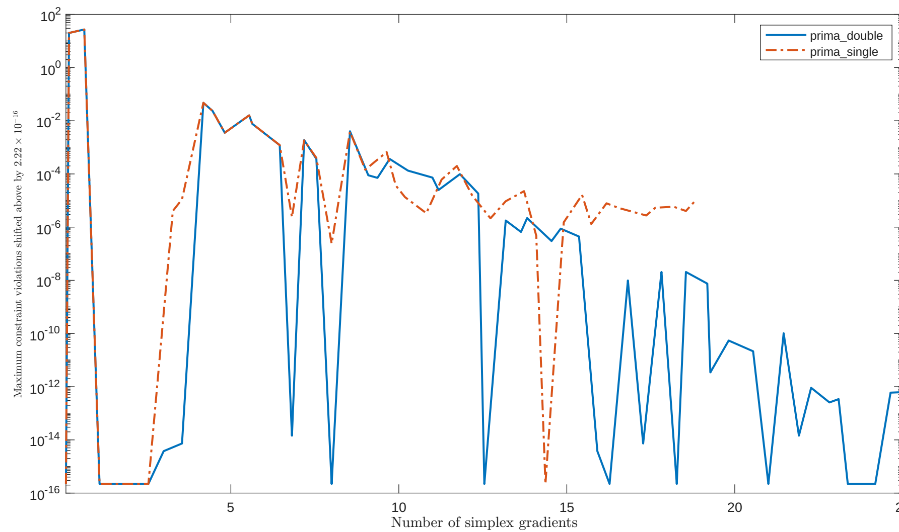
Solving "HS113" with "plain" feature
