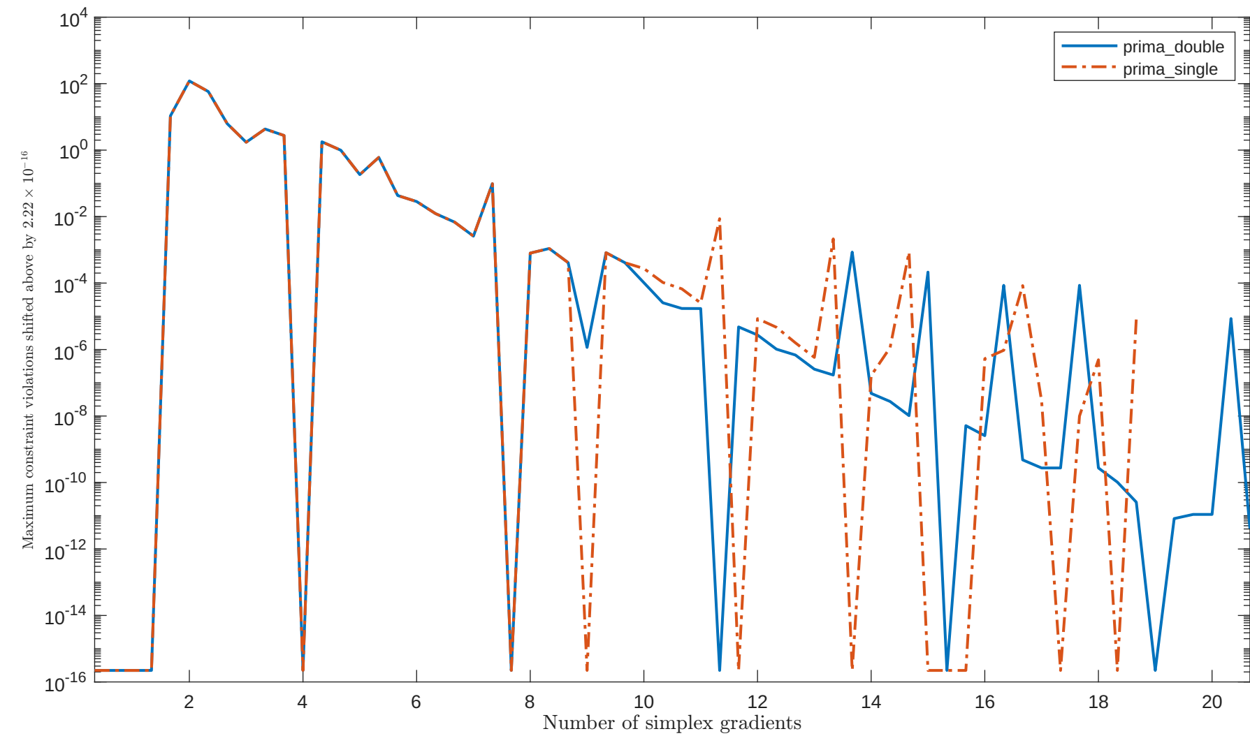
Solving "HS12" with "plain" feature
