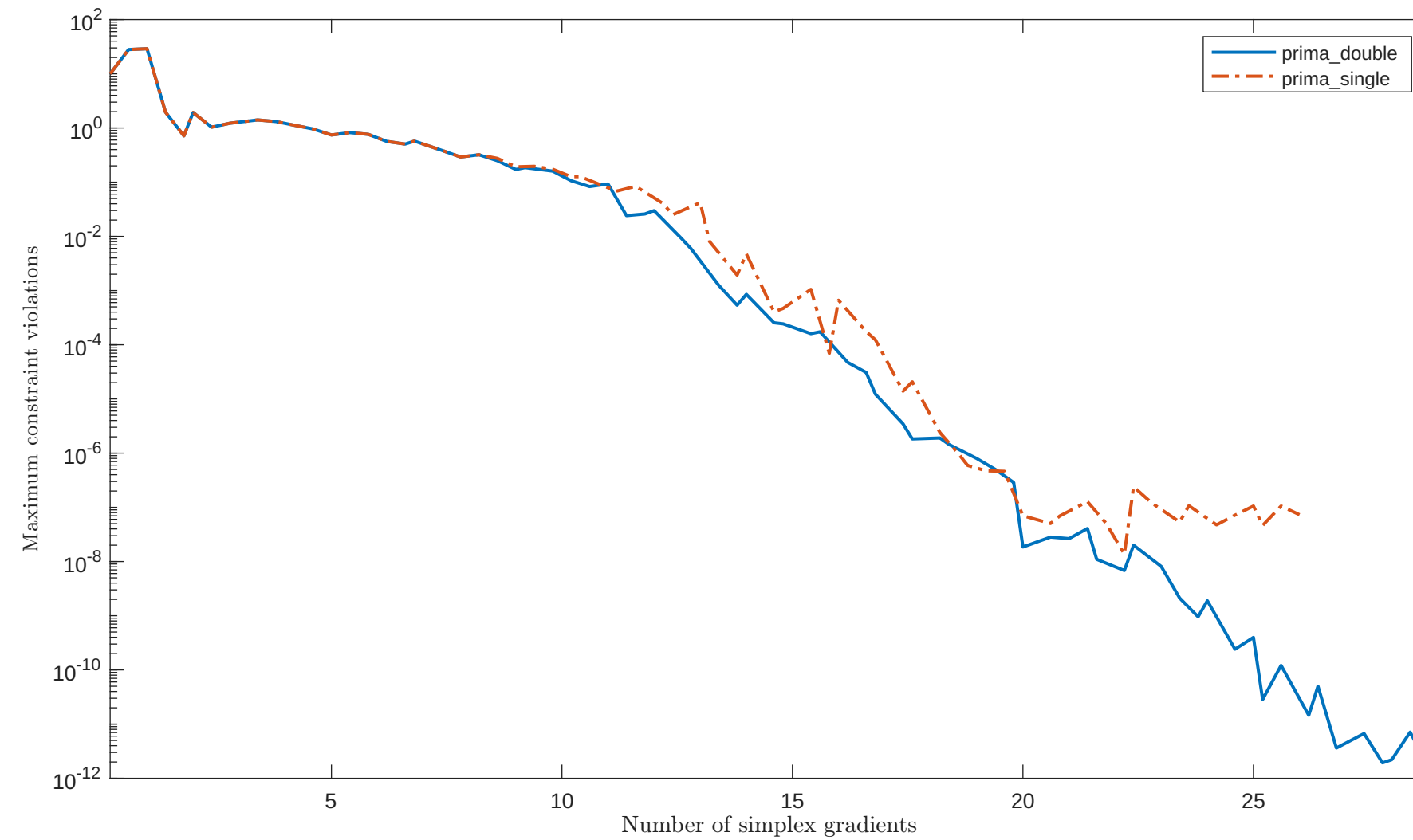
Solving "HS39" with "plain" feature
