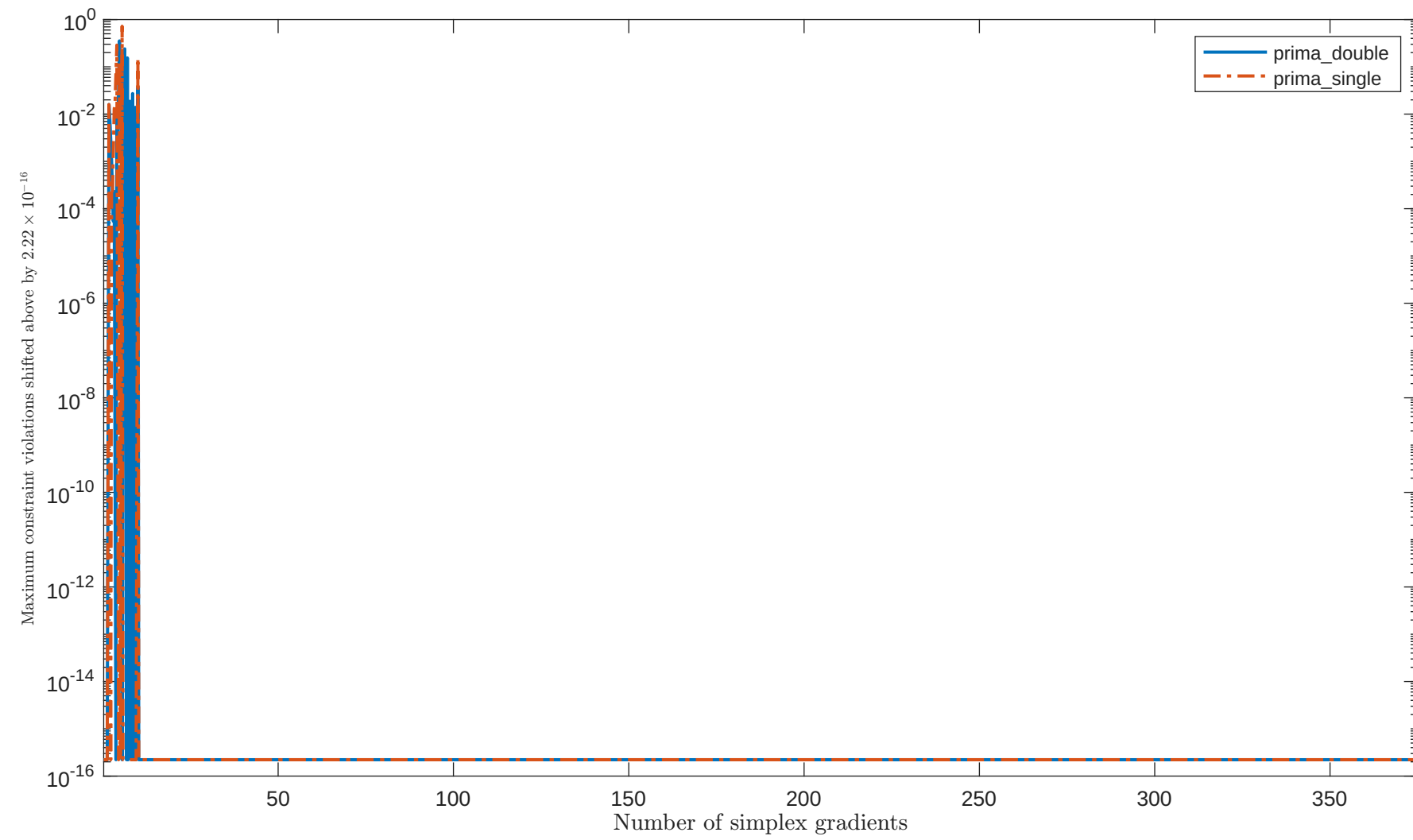
Solving "HS67" with "plain" feature
