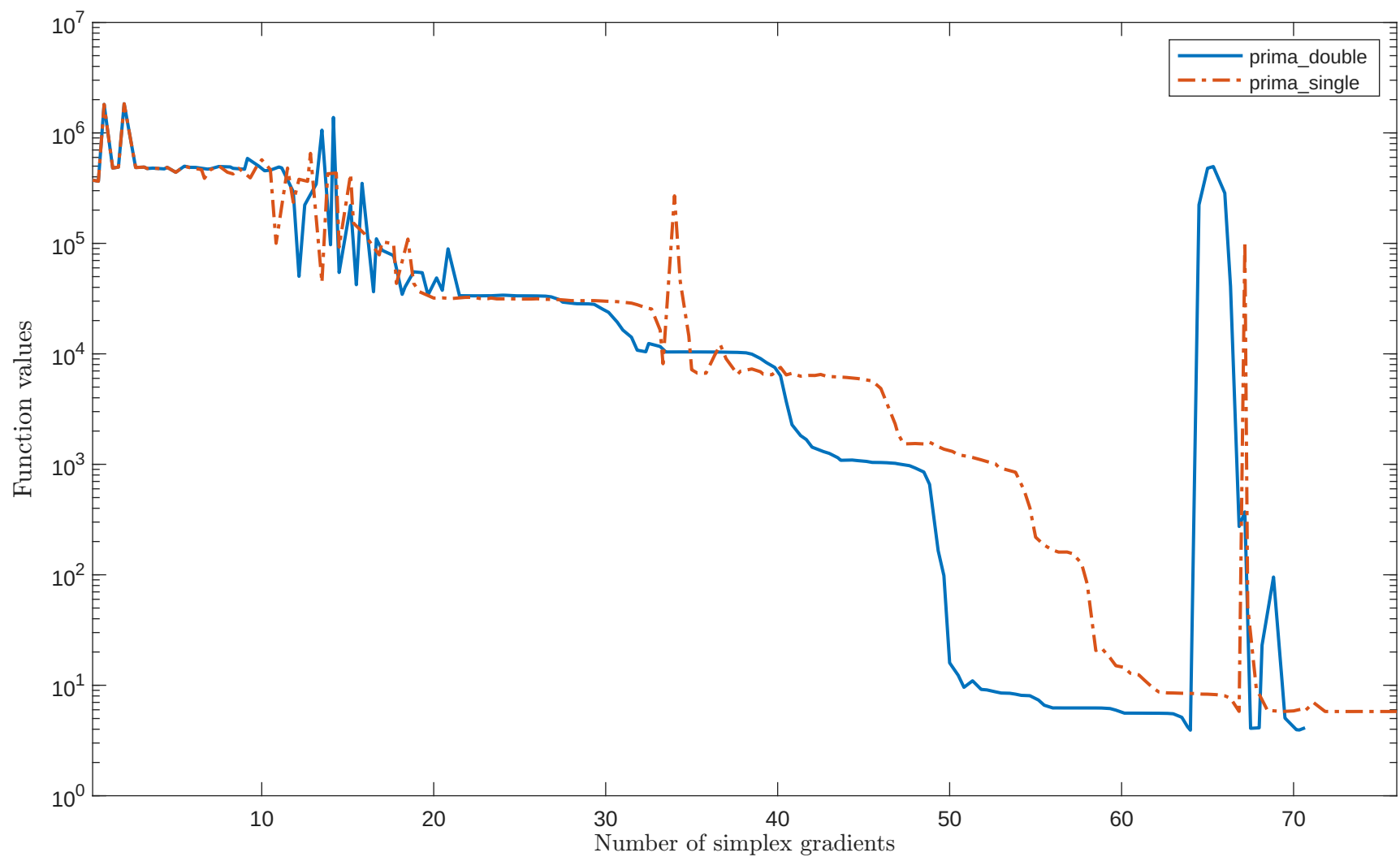
Solving “KIRBY2LS” with “plain” feature
