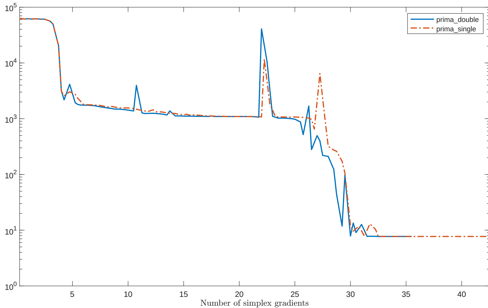
Solving "LSC1LS" with "plain" feature
