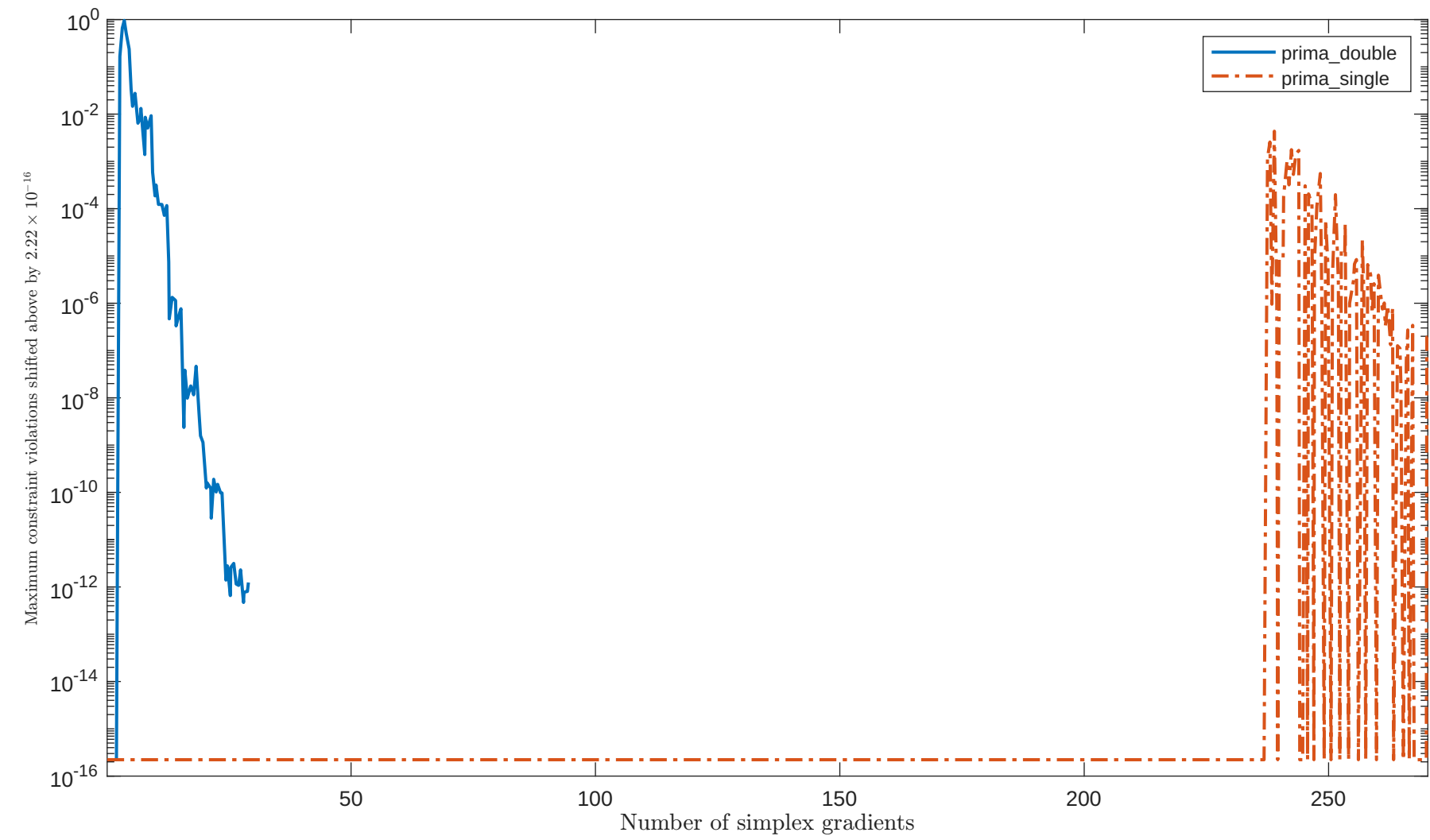
Solving "LUKVLI6" with "plain" feature
