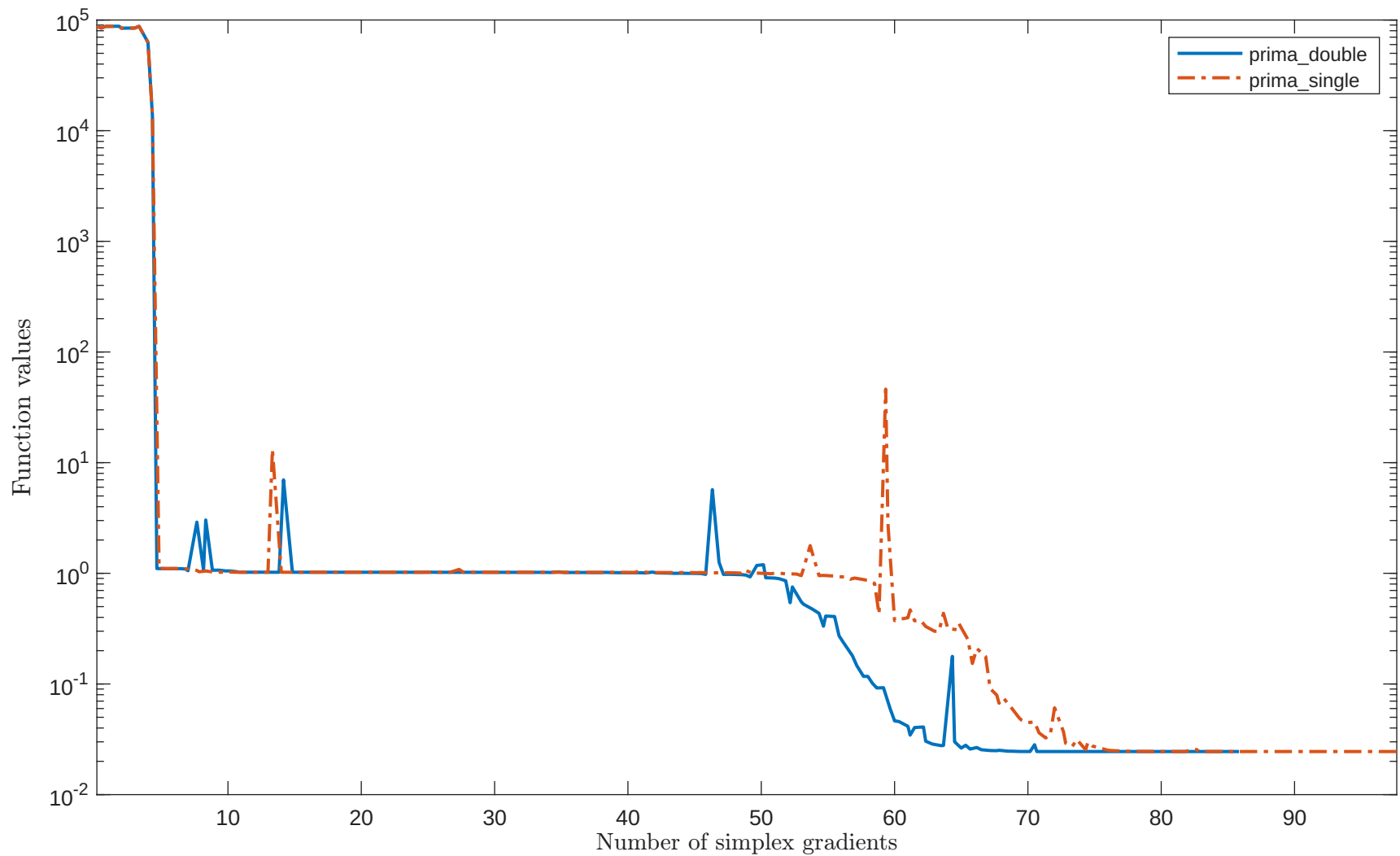
Solving “MGH17SLS” with “plain” feature
