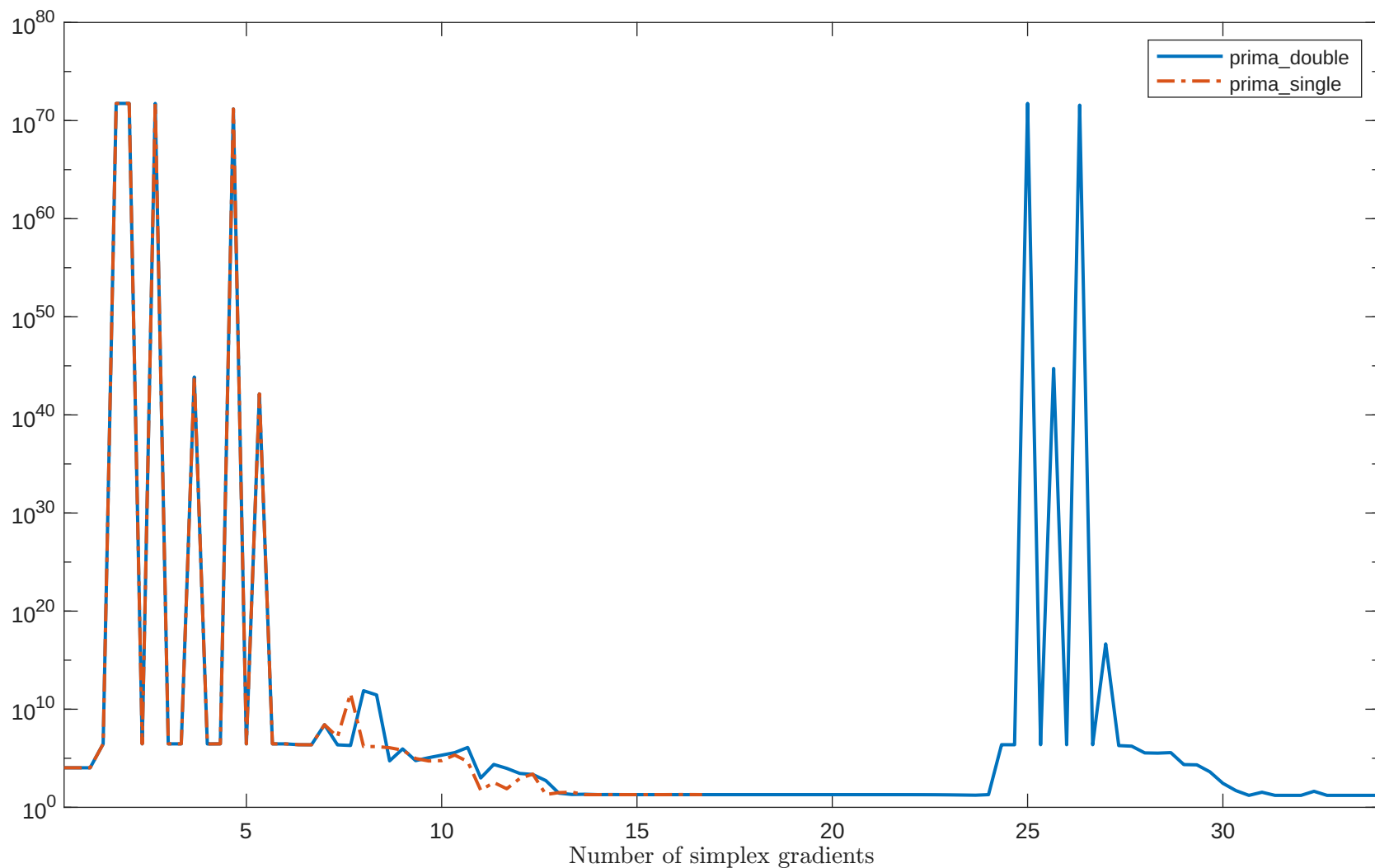
Solving "MISRA1ALS" with "plain" feature
