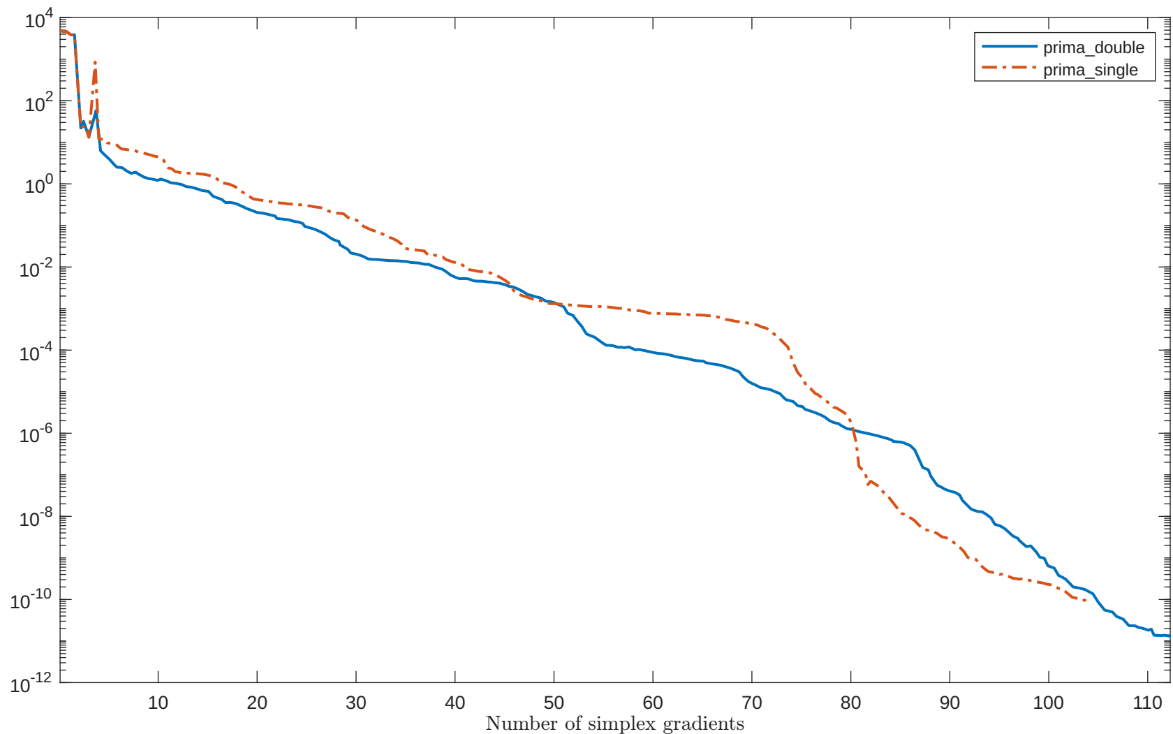
Solving "MODBEALE" with "plain" feature
