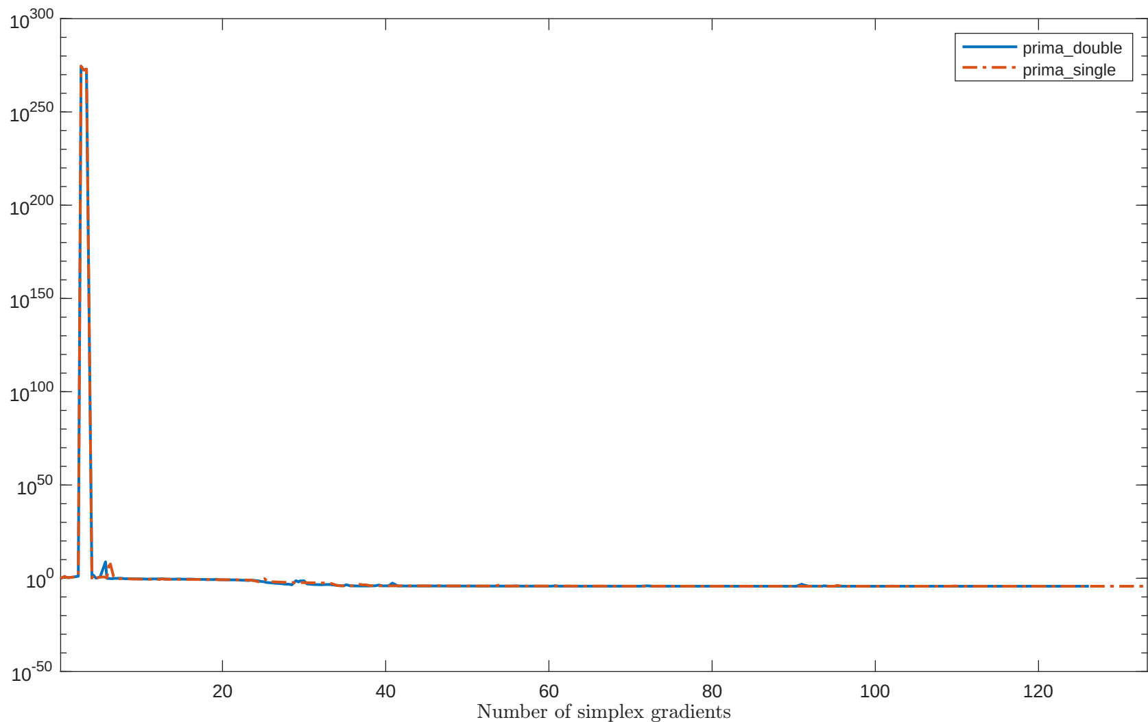
Solving "OSBORNEA" with "plain" feature
