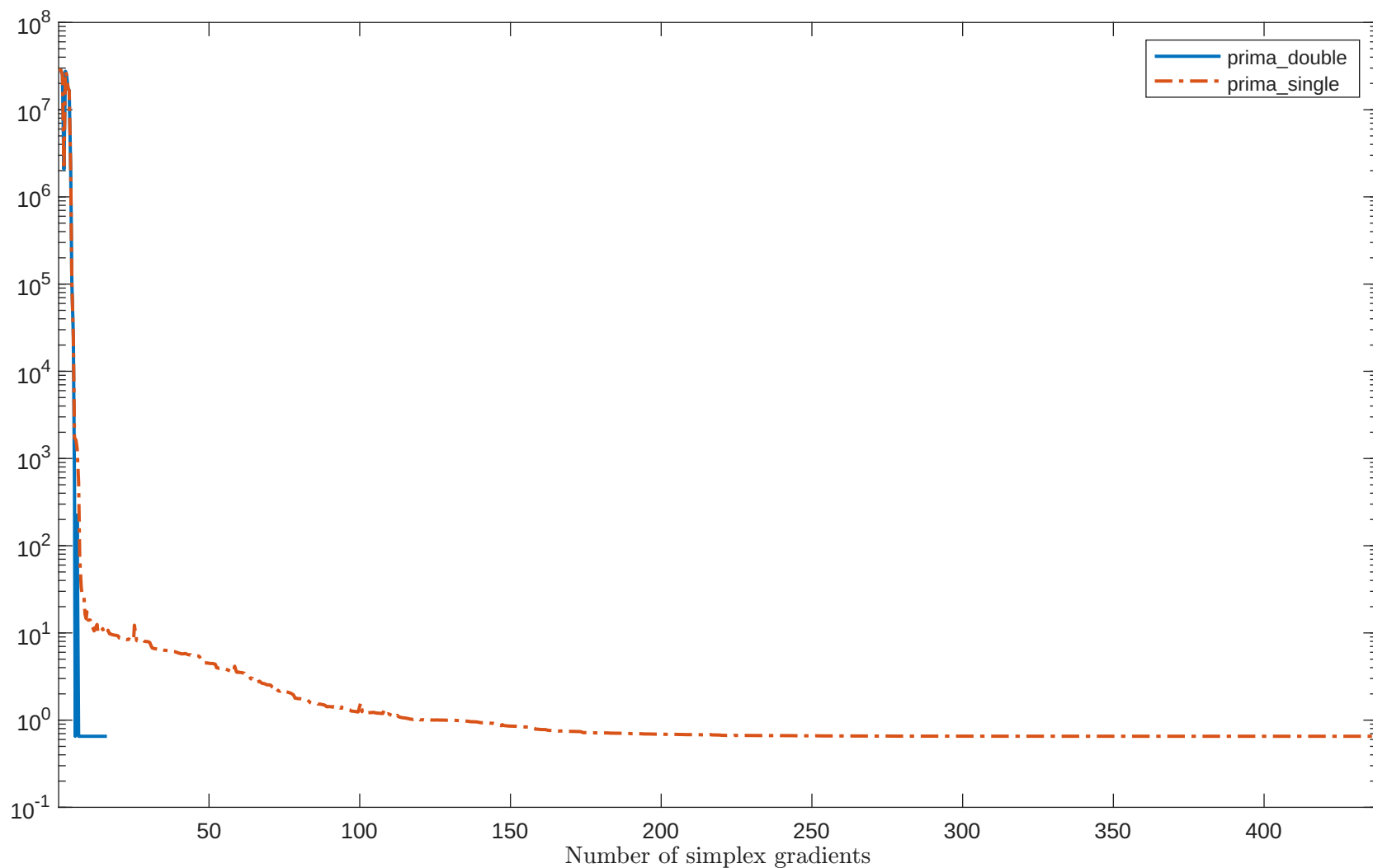
Solving "PALMER1D" with "plain" feature
