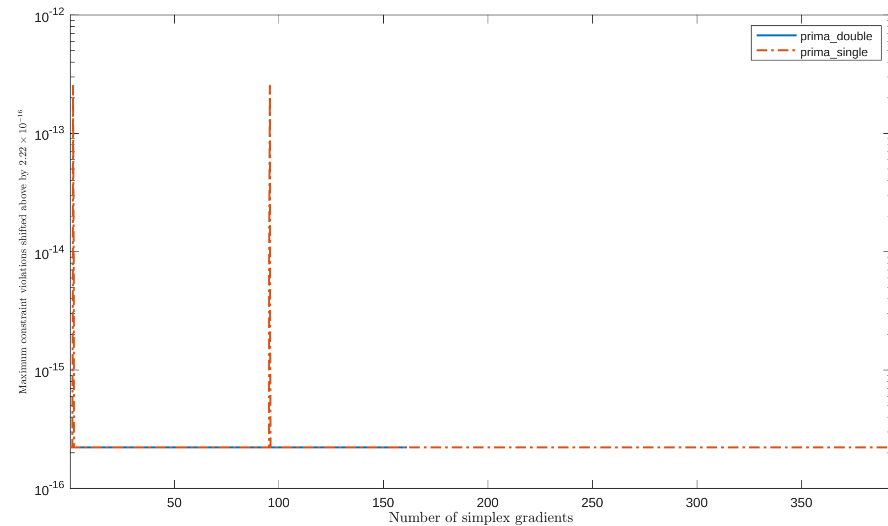
Solving "PALMER2" with "plain" feature
