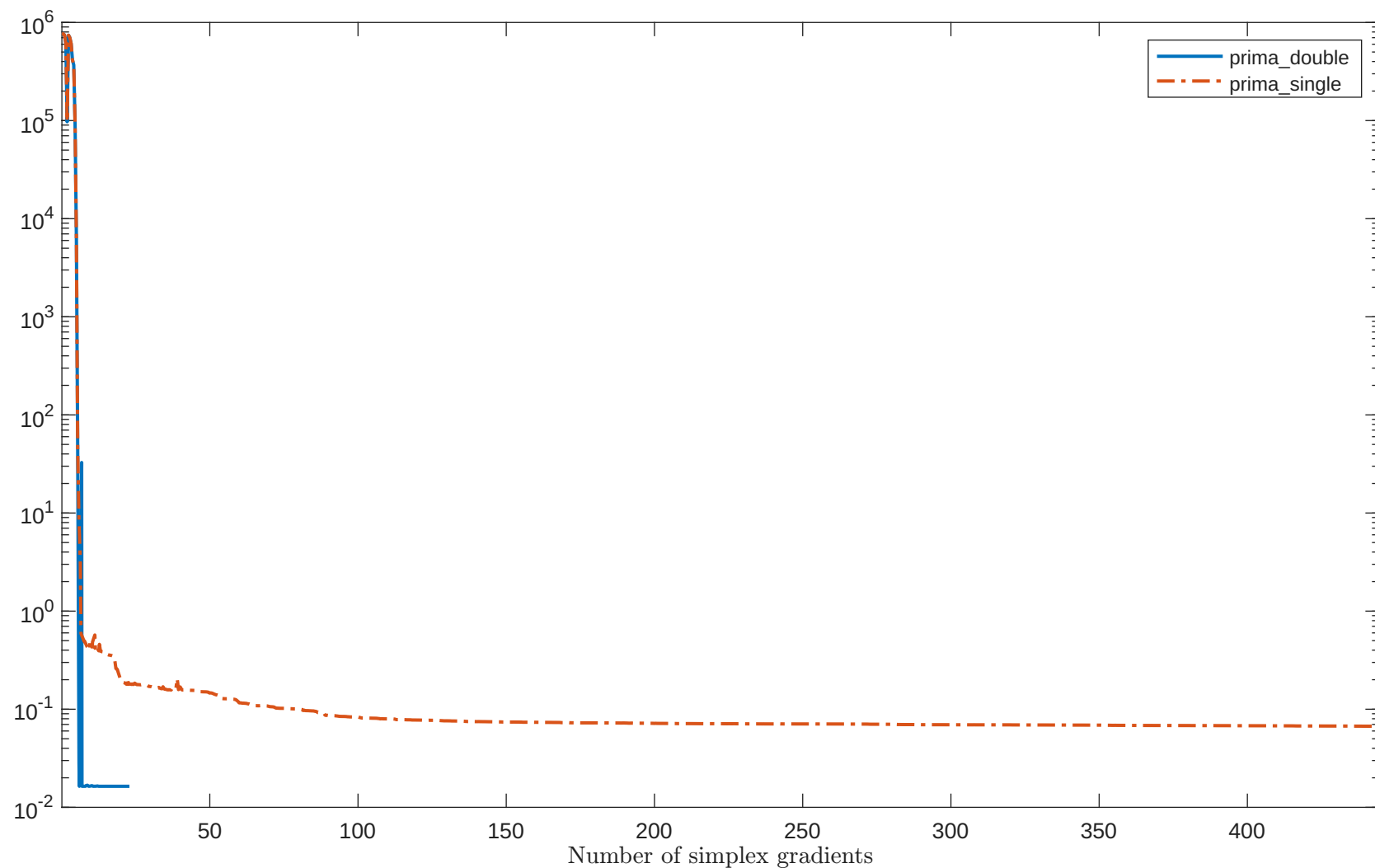
Solving "PALMER6C" with "plain" feature
