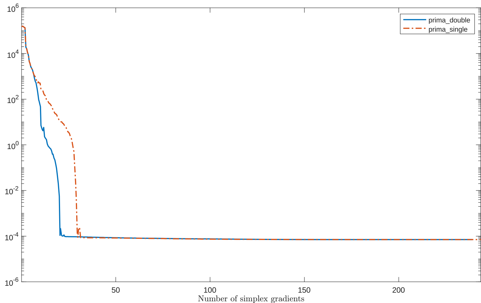
Solving "PENALTY1" with "plain" feature
